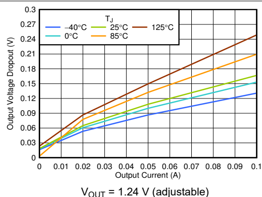
Figure 6-10. V_{DO(OUT)} vs I_{OUT}
