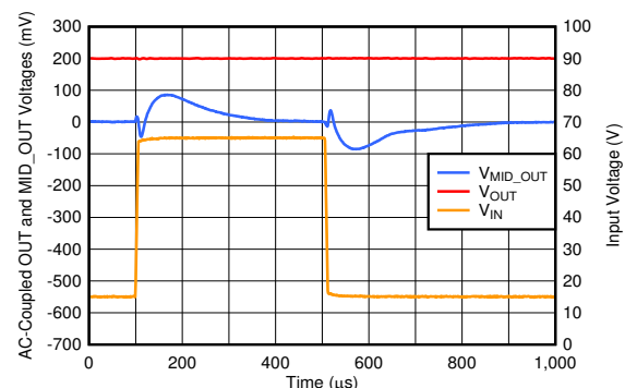
Line Transient With V_{MID\_OUT} = 12\text{ V} , V_{OUT} = 3.3\text{ V} , I_{OUT} = 50\text{ mA}
