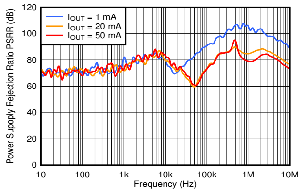
Figure 6-37. OUT PSRR vs Frequency and I_{OUT}
