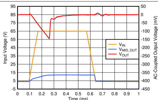
Figure 6-21. Line Transient
