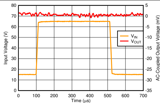
Figure 6-16. Line Transient
