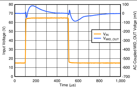
Figure 8-2. TPS7A43 Line Transient: 15 V to 65 V
