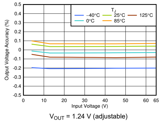
Figure 6-2. V_{\text{OUT}} Accuracy vs V_{\text{IN}}
