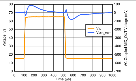
Figure 6-15. Line Transient
