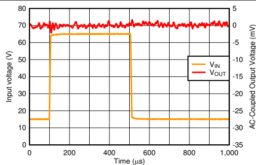
Figure 6-14. Line Transient
