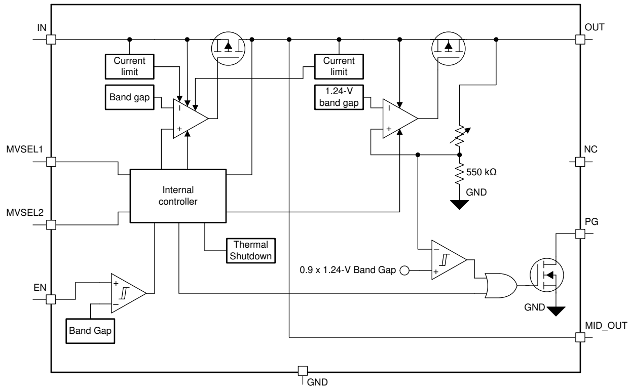
Figure 7-2. Fixed Version
