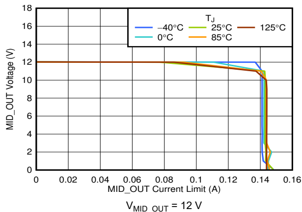
Figure 6-5. V_{\text{MID\_OUT}} vs I_{\text{CL(MID\_OUT)}}
