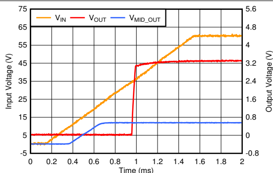
Figure 6-13. Slow Start-Up
