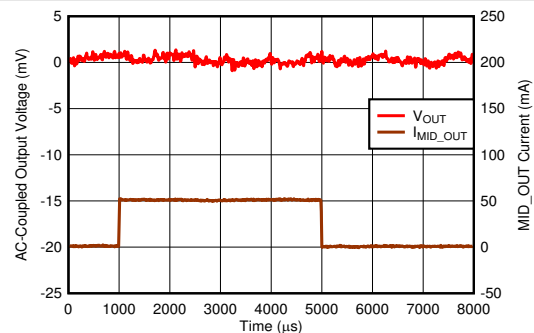
Figure 6-32. Load Transient (MID_OUT)
