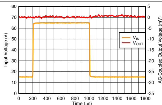
Figure 6-20. Line Transient
