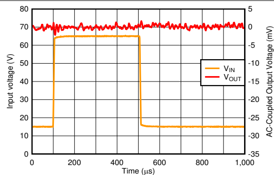
Figure 8-3. TPS7A43 Line Transient: 15 V to 65 V (Zoom on V OUT )
