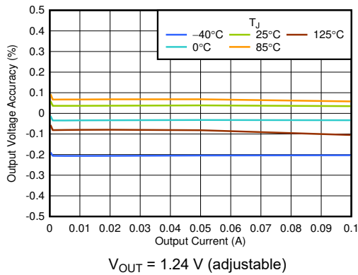
Figure 6-1. V_{\text{OUT}} Accuracy vs I_{\text{OUT}}
