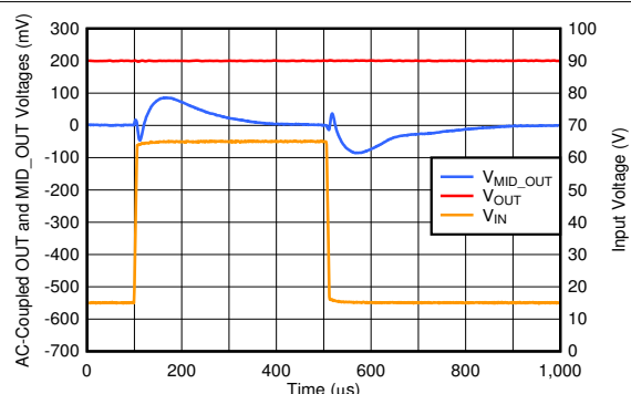
Figure 6-14. Line Transient
