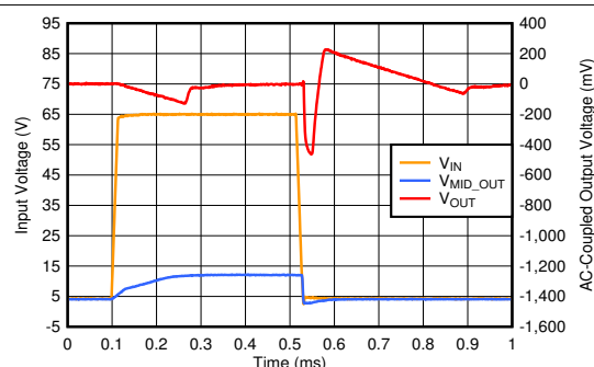
Figure 6-22. Line Transient
