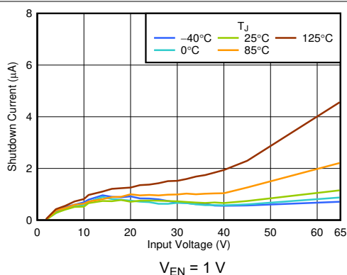
Figure 6-9. I_{SHUTDOWN} vs V_{IN}
