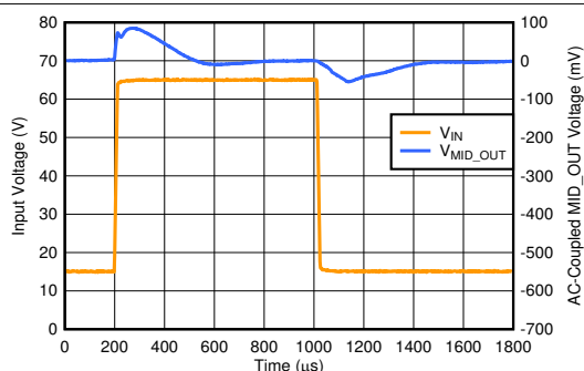
Figure 6-19. Line Transient
