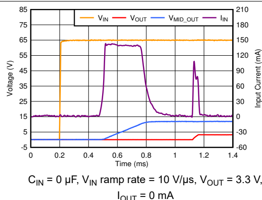
Figure 6-12. Fast Start-Up (Inrush Current)
