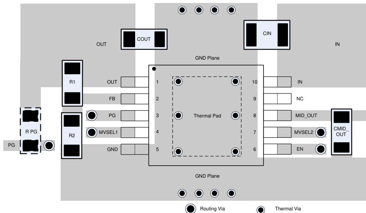
Figure 10-1. Adjustable Version Layout Example
