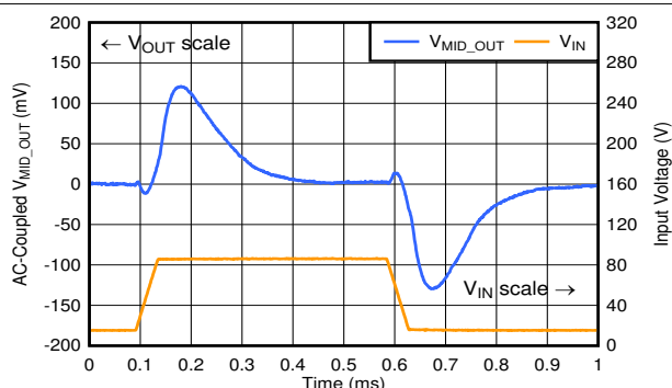
Figure 6-20. Line Transient ( V_{MID\_OUT} in Dropout)
