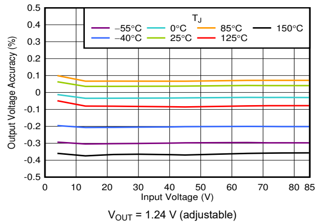
Figure 6-2. V_{\text{OUT}} Accuracy vs V_{\text{IN}}
