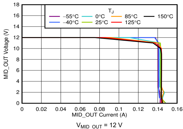
Figure 6-5. V_{\text{MID\_OUT}} vs I_{\text{MID\_OUT}}
