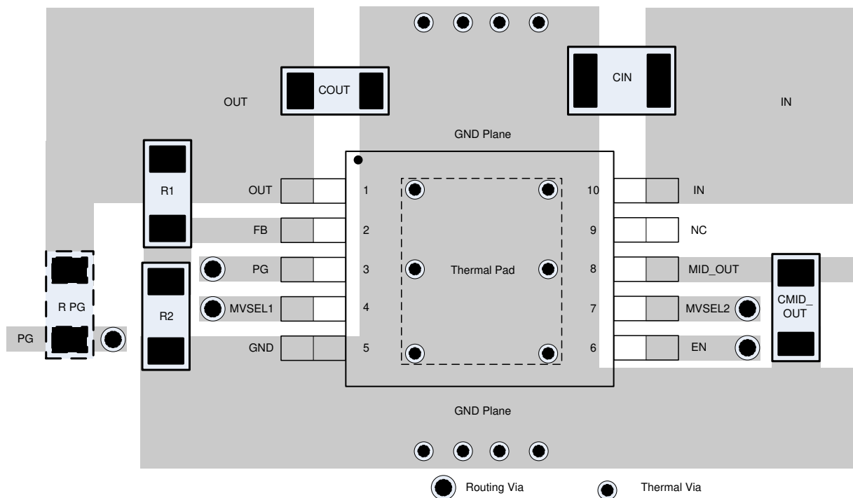
Figure 8-4. Adjustable Version Layout Example
