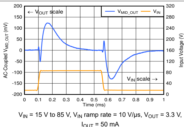
Figure 6-16. Line Transient
