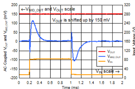
Line Transient With V_{MID\_OUT} = 12\text{ V} , V_{OUT} = 3.3\text{ V} , I_{OUT} = 50\text{ mA}
