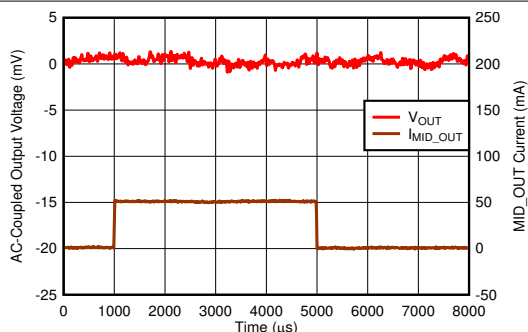
Figure 6-25. Load Transient (Rising Edge)
