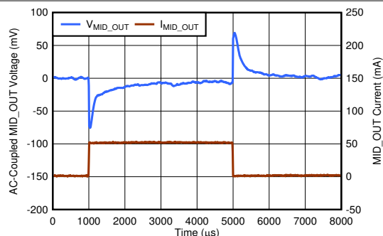
Figure 6-26. Load Transient (MID_OUT)
