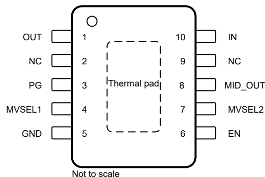
Figure 5-2. DGQ Package (Fixed), 10-Pin HVSSOP (Top View)
