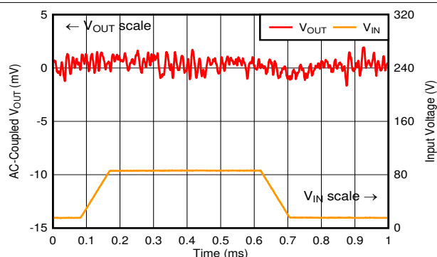
Figure 6-19. Line Transient ( V_{MID\_OUT} in Dropout)
