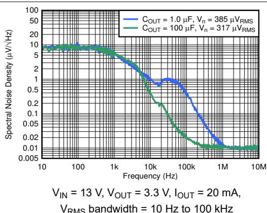
Figure 6-31. Spectral Noise Density vs Frequency and C_{OUT}
