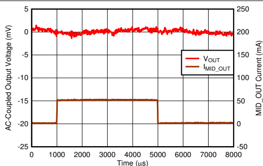
Figure 6-27. Load Transient (MID_OUT)
