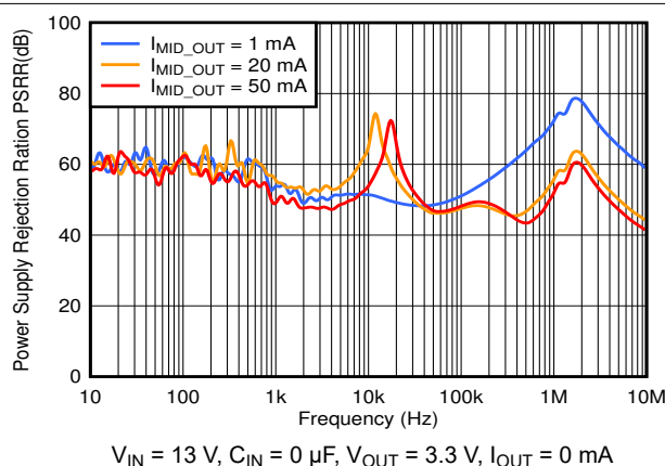
Figure 6-35. MID_OUT PSRR vs Frequency and I_{MID\_OUT}
