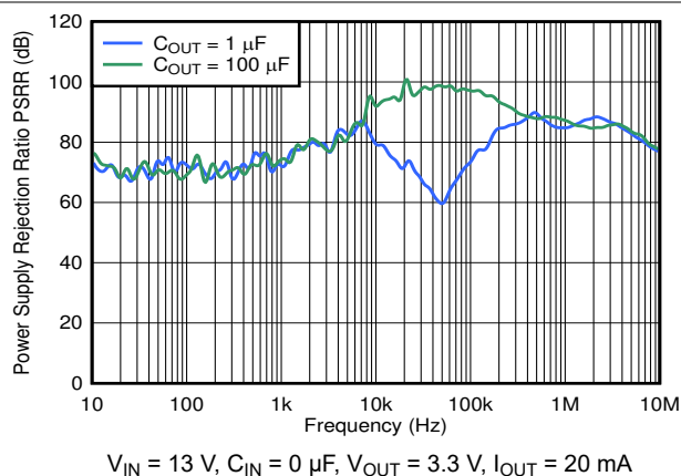
Figure 6-34. OUT PSRR vs Frequency and C_{OUT}
