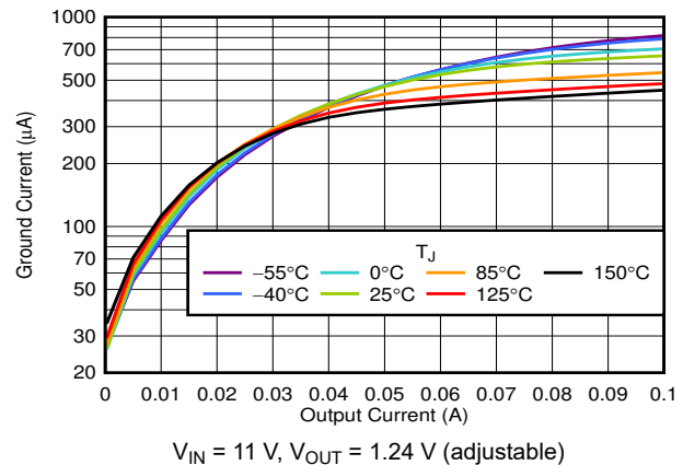
Figure 6-6. I_{\text{GND}} vs I_{\text{OUT}} ( \text{MID\_OUT} in Dropout)
