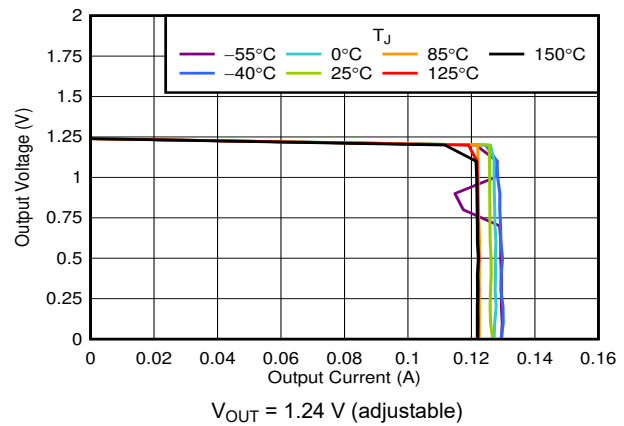
Figure 6-4. V_{\text{OUT}} vs I_{\text{CL(OUT)}}
