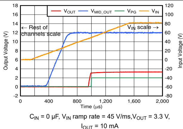
Figure 6-13. Slow Start-Up
