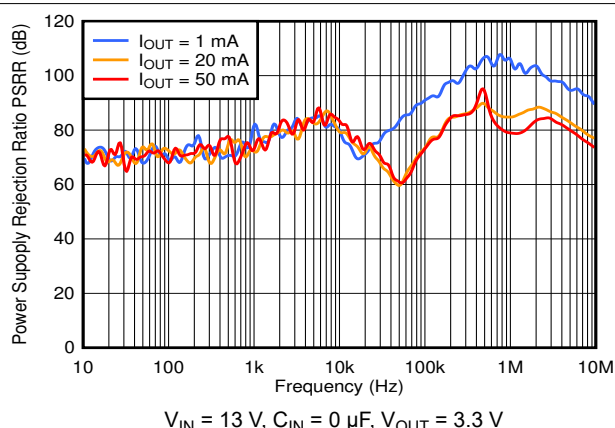
Figure 6-32. OUT PSRR vs Frequency and I_{OUT}
