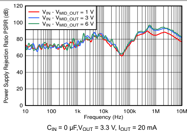
Figure 6-33. OUT PSRR vs Frequency and V_{IN}
