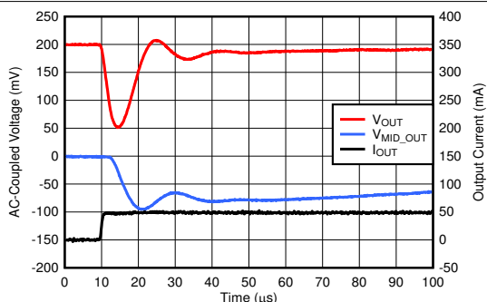
Figure 6-25. Load Transient (Rising Edge)
