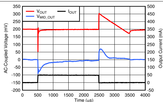
Figure 6-22. Load Transient
