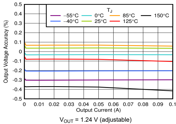
Figure 6-1. V_{\text{OUT}} Accuracy vs I_{\text{OUT}}
