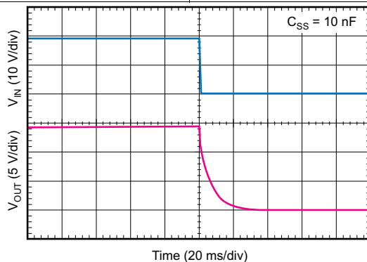
Figure 25. Line Transient
