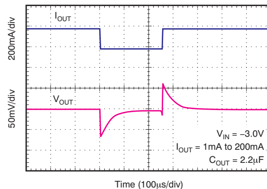
Figure 37. Load Transient Response
