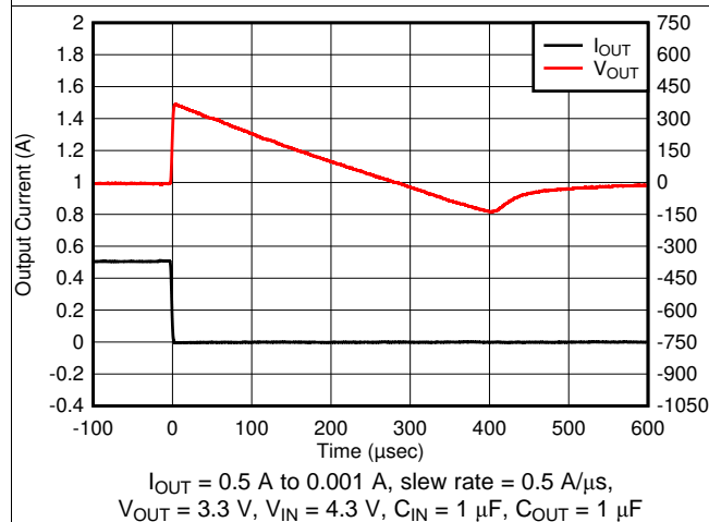
Figure 29. Load Transient
