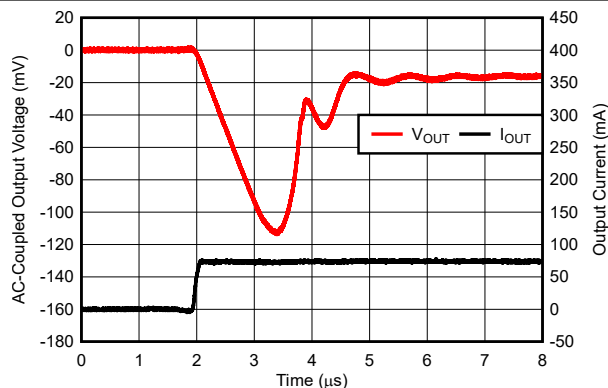
Figure 5-19. Load Transient
