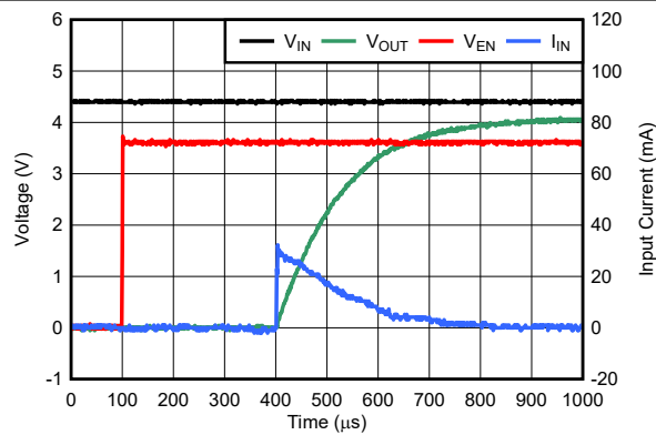
Figure 5-37. Start-Up
