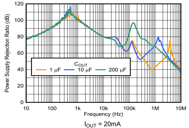
Figure 5-28. PSRR vs Frequency and C_{OUT}
