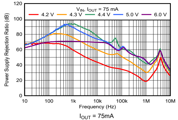
Figure 5-26. PSRR vs Frequency and V_{IN}
