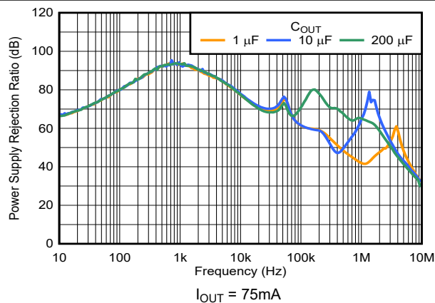
Figure 5-29. PSRR vs Frequency and C_{OUT}
