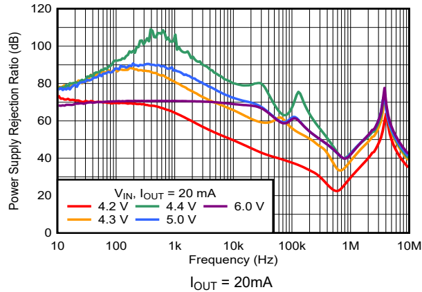
Figure 5-25. PSRR vs Frequency and V_{IN}
