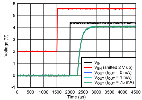
Figure 5-38. Start-Up
