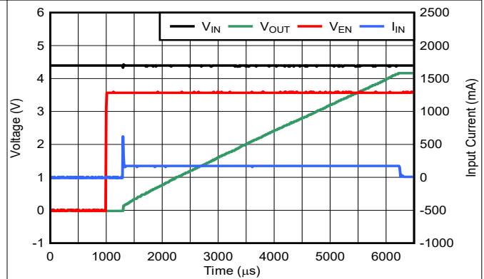
Figure 5-38. Start-Up
