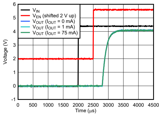
Figure 5-37. Start-Up
