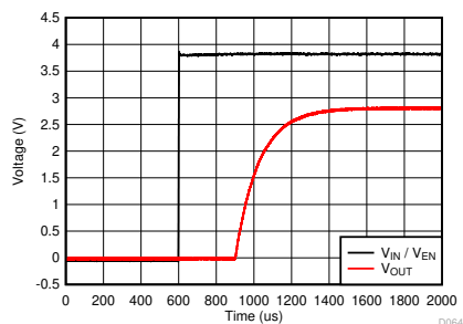
Figure 7-5. Start-Up
