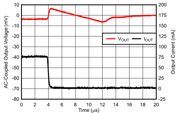
Figure 5-20. Load Transient
