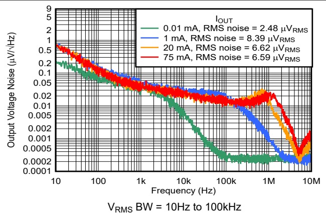
Figure 5-30. Noise vs Frequency and I_{OUT}
