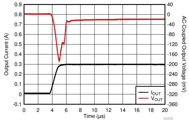
Figure 5-38. Load Transient
