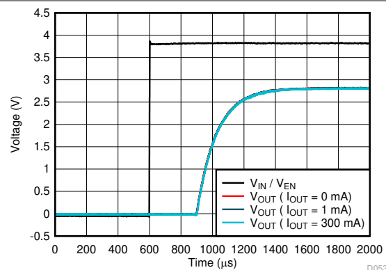
Figure 5-62. Start-Up
