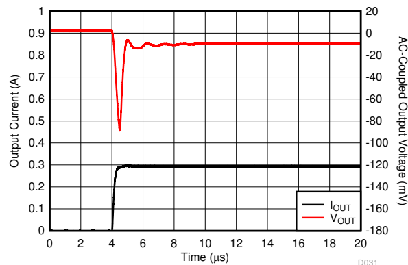
Figure 5-36. Load Transient
