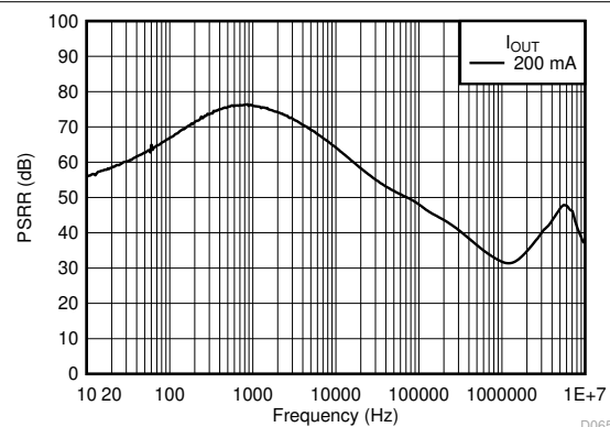
Figure 7-6. PSRR
