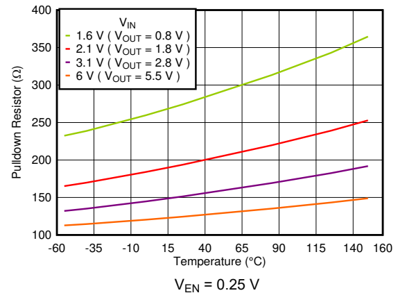
Figure 5-32. Output Pulldown Resistor vs Temperature
