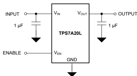
Simplified Schematic
