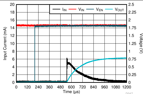
Figure 5-64. Start-Up
