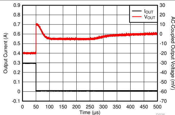
Figure 5-39. Load Transient
