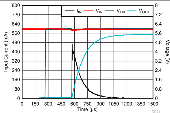
Figure 5-68. Inrush Current
