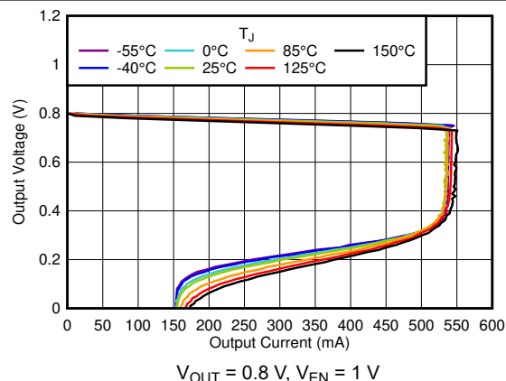
Figure 5-28. Current Limit
