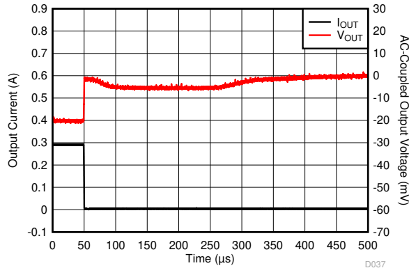
Figure 5-37. Load Transient
