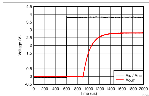
Figure 7-5. Start-Up
