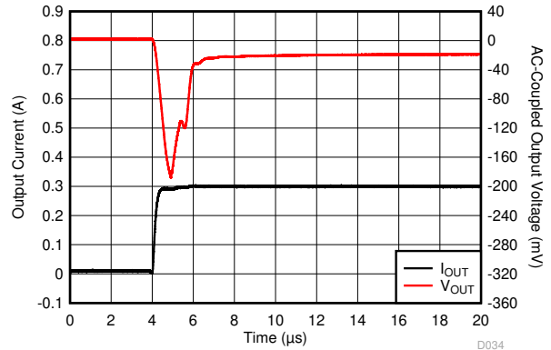
Figure 5-38. Load Transient
