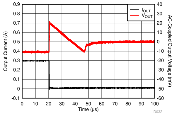
Figure 5-37. Load Transient
