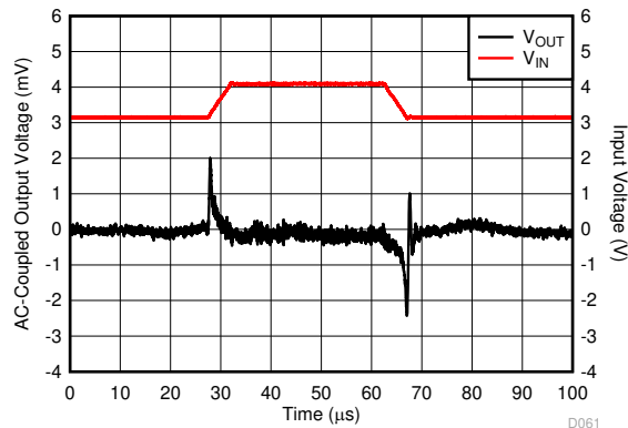
Figure 5-43. Line Transient
