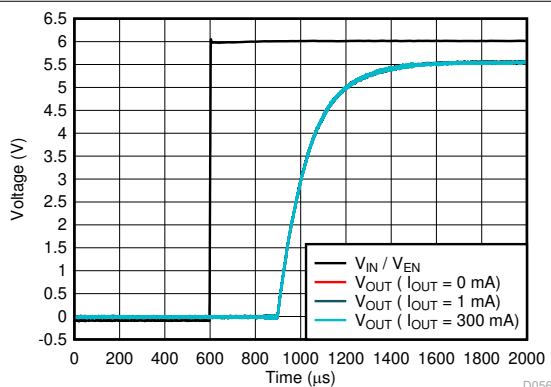
Figure 5-63. Start-Up
