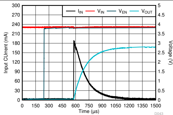
Figure 5-67. Inrush Current
