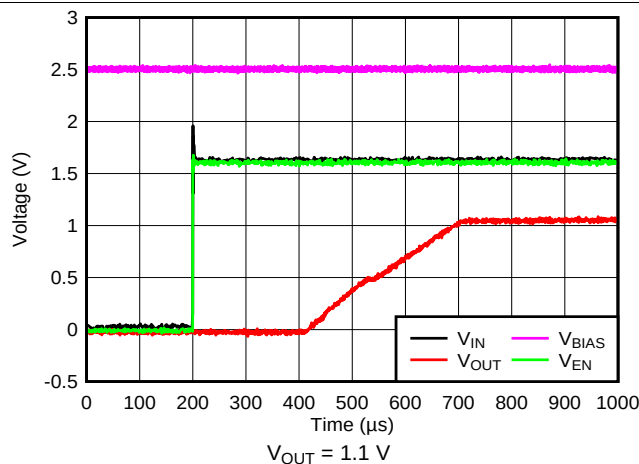
Figure 21. Startup With V_{EN} = V_{IN}
