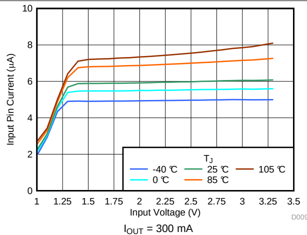
Figure 19. I_Q ( V_{IN} ) Over Temperature
