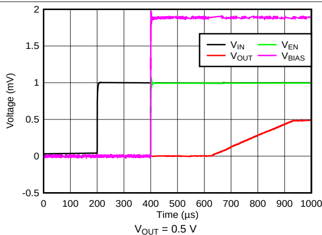
Figure 23. Startup With V_{EN} and V_{BIAS} Powering Up Simultaneously
