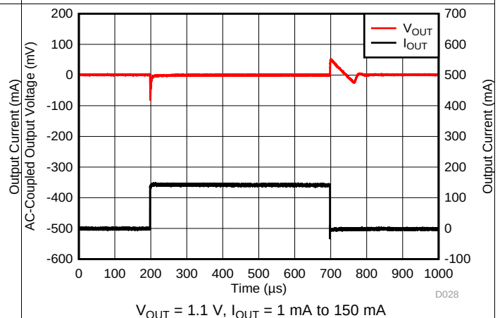
Figure 10. I_{OUT} Transient
