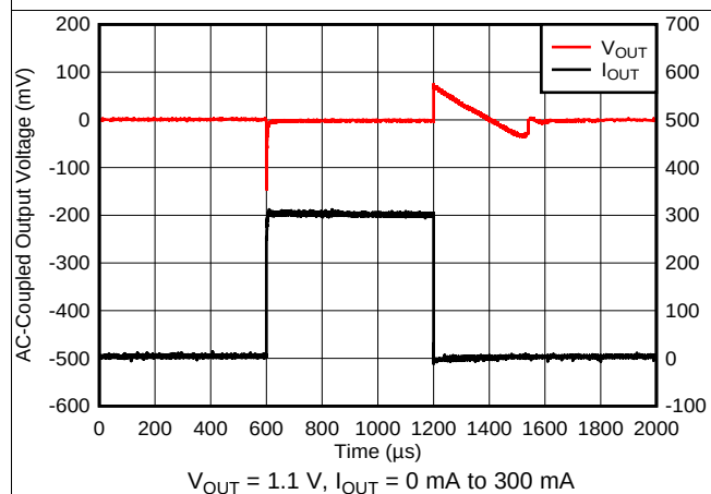
Figure 11. I_{OUT} Transient
