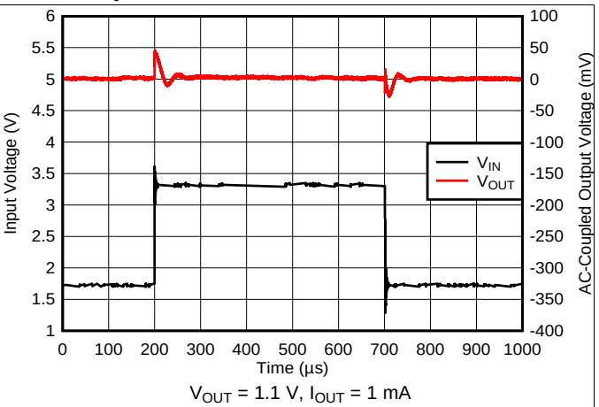
Figure 14. V_{IN} Transient
