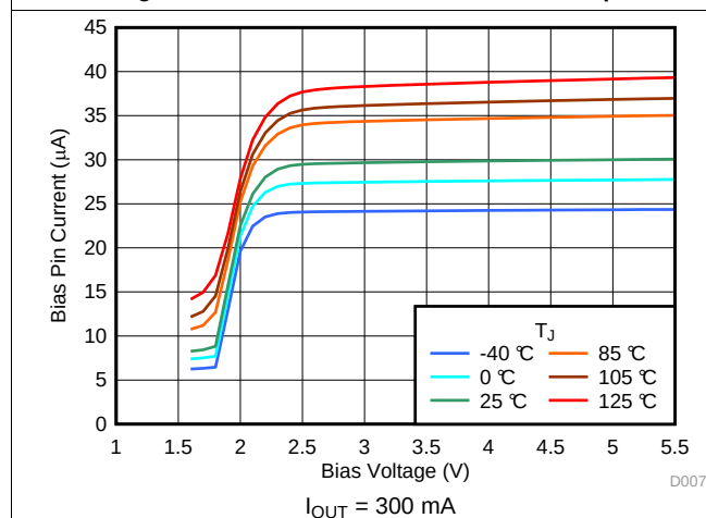
Figure 17. I_Q (V_{BIAS}) Over Temperature
