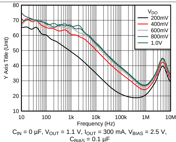
Figure 29. PSRR vs Frequency and V_{DO}
