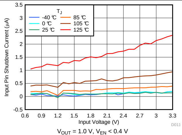
Figure 20. I_{SHDN} ( V_{IN} ) Over Temperature
