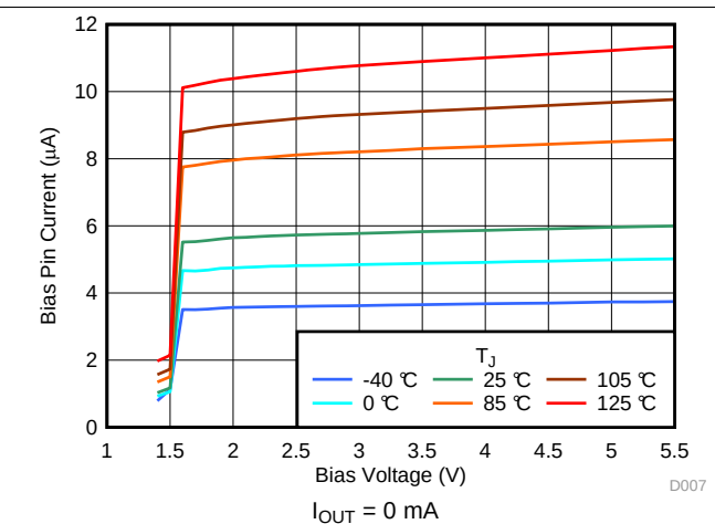
Figure 16. I_Q (V_{BIAS}) Over Temperature
