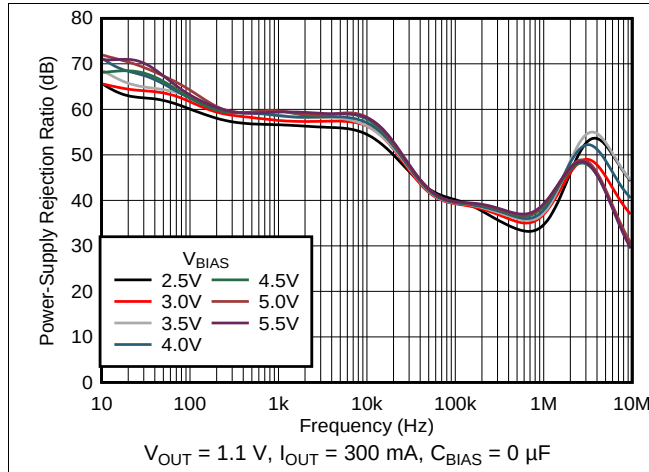
Figure 31. V_{BIAS} PSRR vs Frequency and V_{BIAS}
