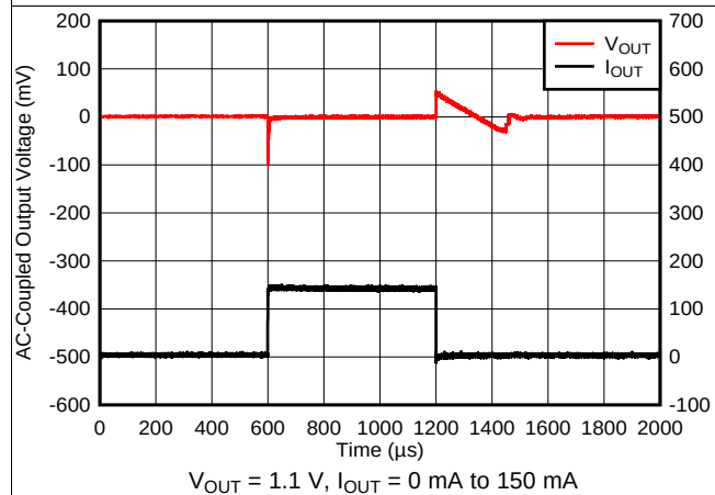
Figure 9. I_{OUT} Transient
