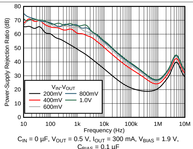
Figure 30. PSRR vs Frequency and V_{DO}
