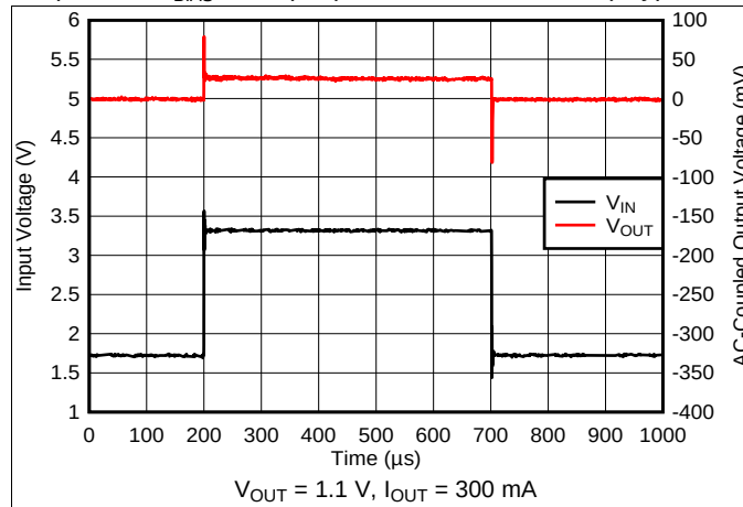
Figure 13. V_{IN} Transient
