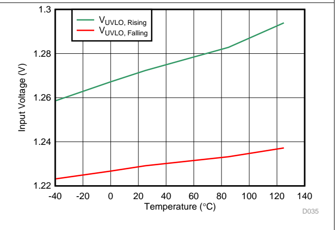
Figure 46. UVLO V_{IN} Rising and Falling Thresholds vs Temperature
