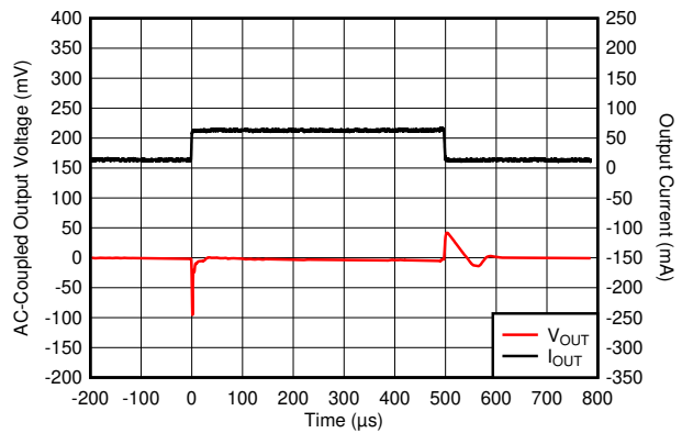
Figure 6-12. I_{OUT} Transient From 1 mA to 50 mA
