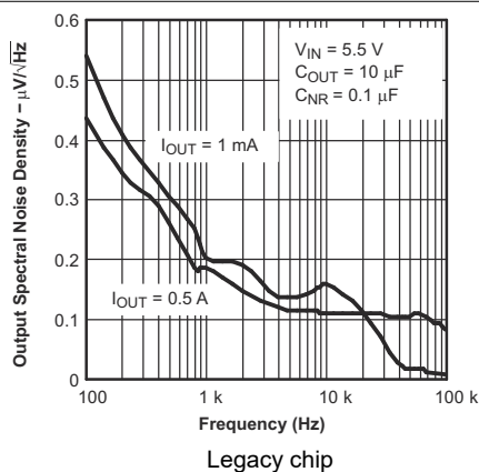
Figure 5-9. TPS79530 Output Spectral Noise Density vs Frequency
