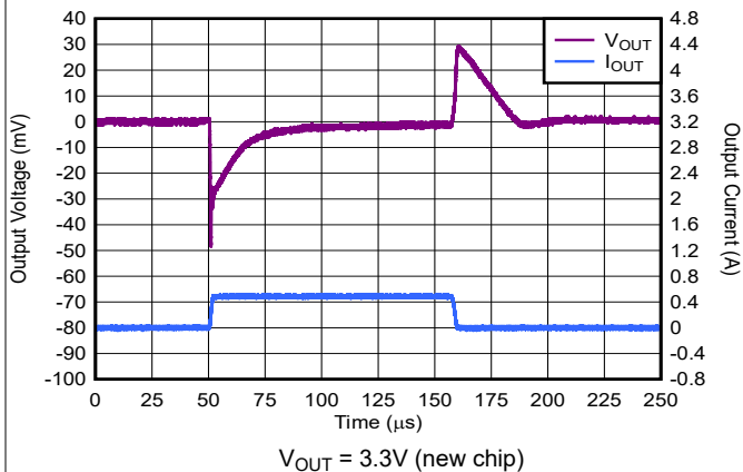
Figure 5-26. TPS795 Load Transient Response
