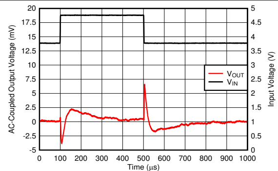
Figure 6-16. Line Transient
