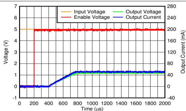
Figure 6-28. Start-Up Inrush Current With C_{OUT} = 1\text{ }\mu\text{F}
