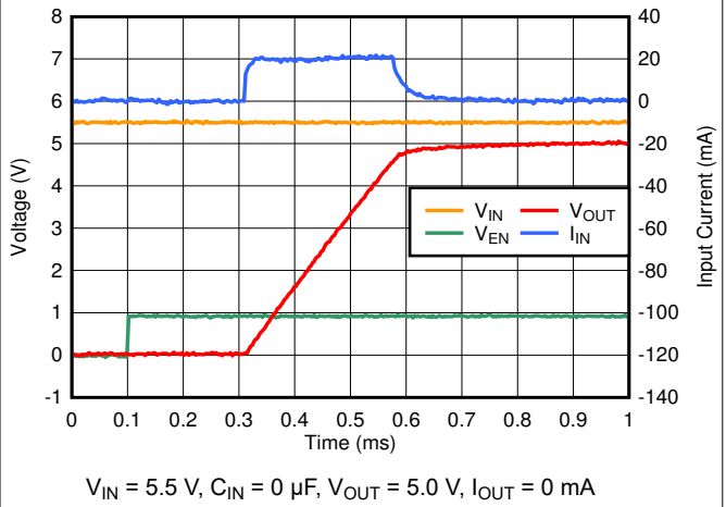
Figure 6-32. Startup Inrush Current With C_{OUT} = 1\ \mu\text{F}
