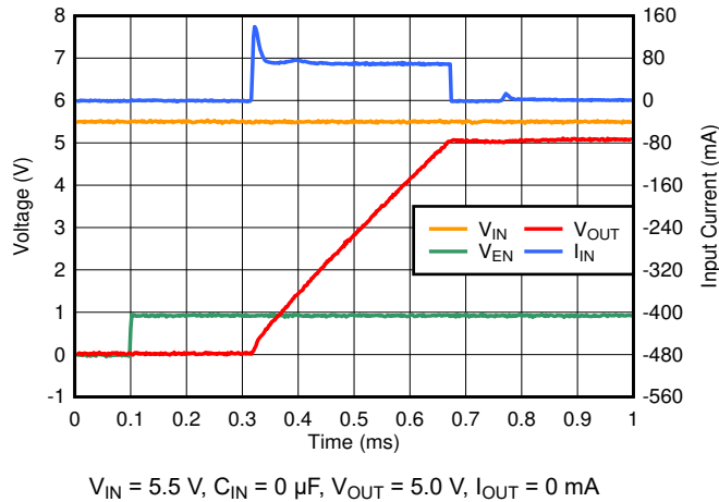
Figure 6-33. Startup Inrush Current With C_{OUT} = 4.7\ \mu\text{F}
