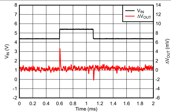
Figure 7-7. TPS77015 Line Transient Response (Legacy Chip)
