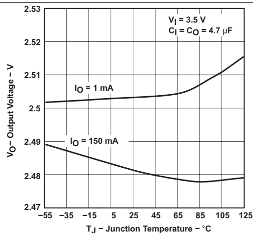
Figure 4. TPS76325 Output Voltage vs Junction Temperature
