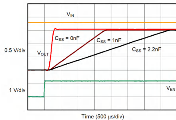
Figure 6-44. Turn-On Response
