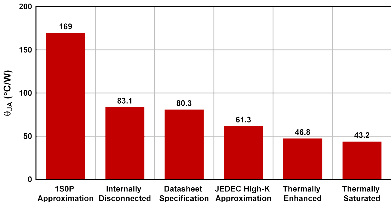
Figure 7-8. TPS746-Q1 (WSON) R_{\theta JA} vs Board Layout
