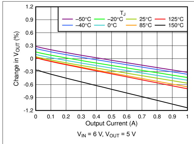
Figure 5-13. 5-V Load Regulation vs I_{OUT}
