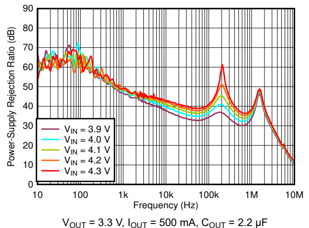
Figure 5-32. PSRR vs Frequency and V_{IN}
