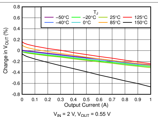
Figure 5-12. 0.55-V Load Regulation vs I_{OUT}
