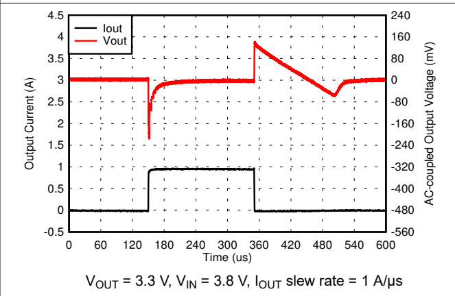
Figure 5-28. 1-mA to 1-A Load Transient (3.3 V)
