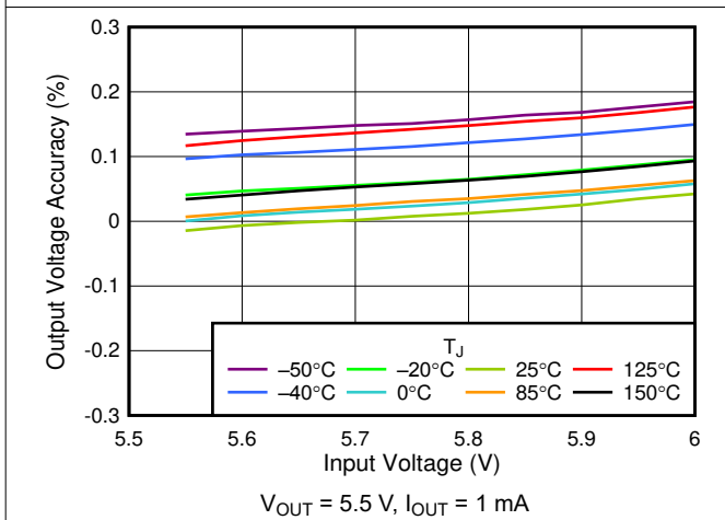
Figure 5-3. 5.5-V Line Regulation vs V_{IN}
