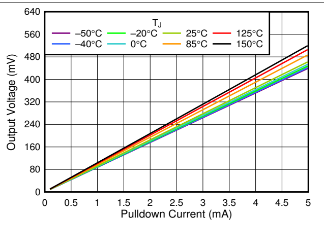
Figure 5-14. V_{OUT} vs I_{OUT} Pulldown Resistor
