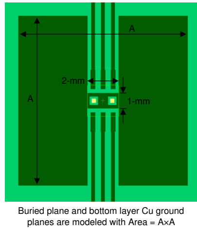
Figure 7-7. Board Parameters Used for Simulation
