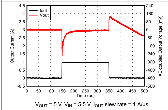
Figure 5-27. 1-mA to 1-A Load Transient (5 V)
