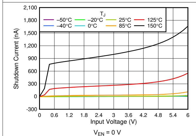
Figure 5-9. I_{SHDN} vs V_{IN}
