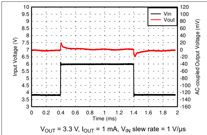
Figure 5-25. 3.3-V Line Transient
