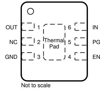
Figure 4-2. DRV Package, 6-Pin Fixed WSON (Top View)
