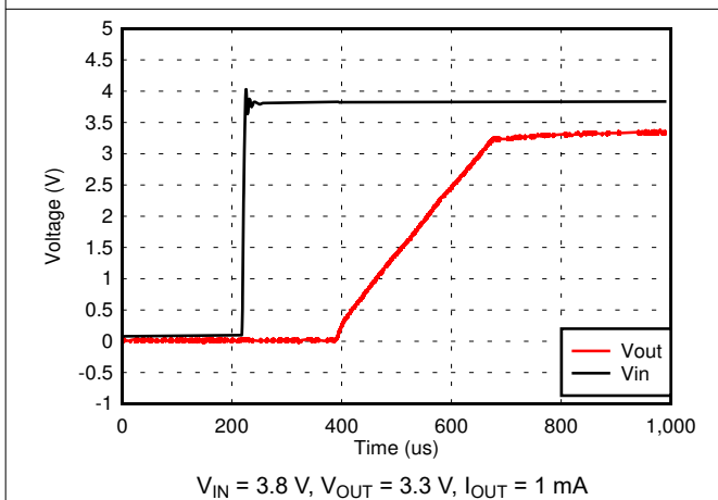
Figure 5-29. V_{IN} Power-Up
