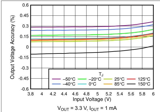
Figure 5-1. 3.3-V Line Regulation vs V_{IN}
