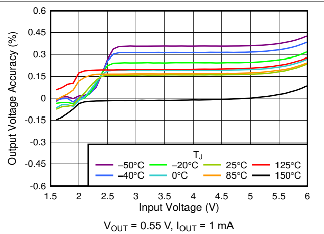
Figure 5-2. 0.55-V Line Regulation vs V_{IN}
