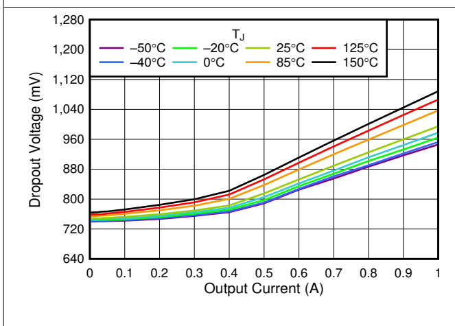
Figure 5-5. 0.55-V Dropout Voltage vs I_{OUT}
