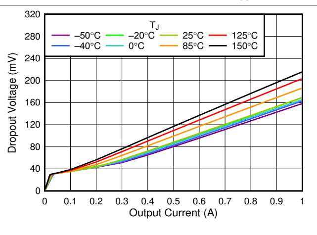
Figure 5-6. 5.5-V Dropout Voltage vs I_{OUT}
