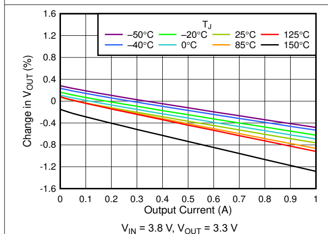
Figure 5-11. 3.3-V Load Regulation vs I_{OUT}
