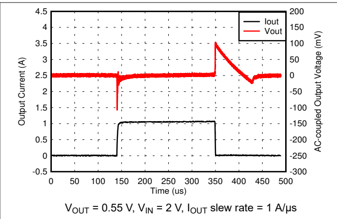
Figure 5-26. 1-mA to 1-A Load Transient (0.55 V)
