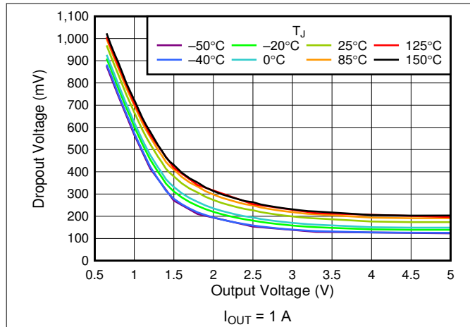
Figure 5-7. V_{DO} vs V_{OUT}
