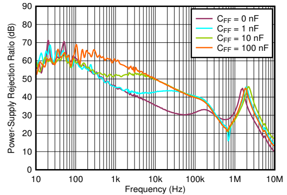
Figure 5-38. PSRR vs Frequency and C_{FF}
