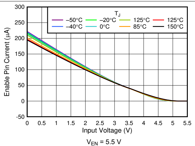
Figure 5-22. I_{EN} vs V_{IN}
