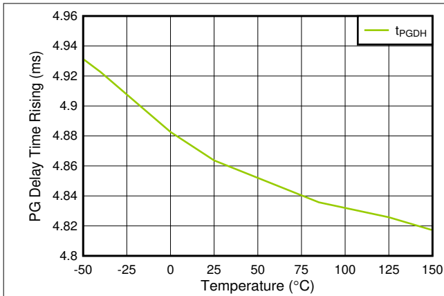
Figure 5-19. t_{PGDH} vs Temperature (For TPS746B Only)
