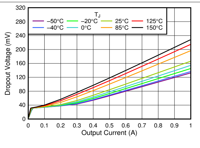
Figure 5-4. 3.3-V Dropout Voltage vs I_{OUT}
