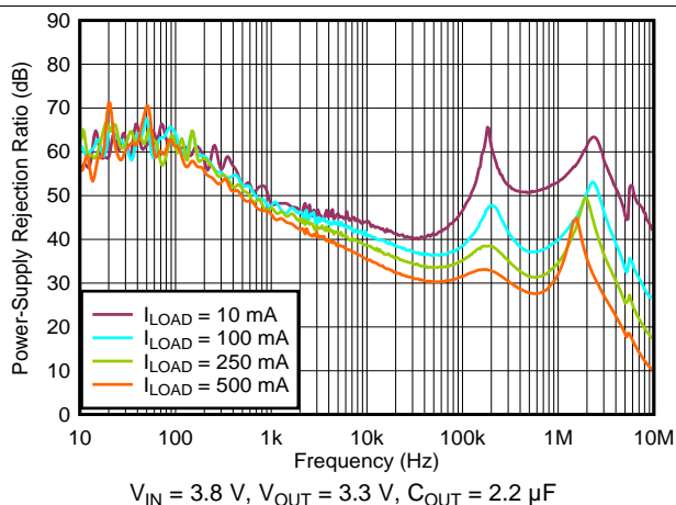
Figure 38. PSRR vs Frequency and I_{LOAD}
