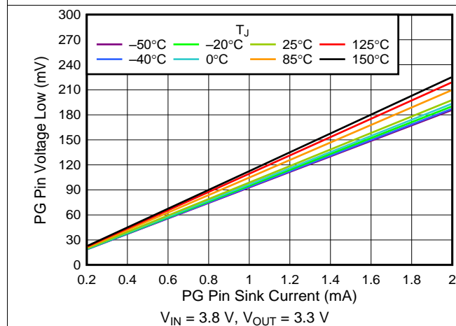
Figure 17. V_{OL(PG)} vs PG Pin Sink Current
