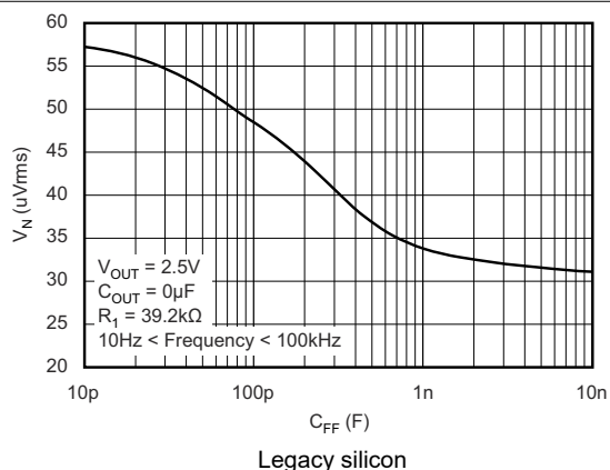
Figure 5-29. TPS73701 RMS Noise Voltage vs C_{FB}
