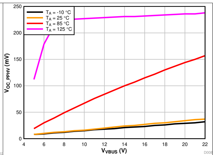
Figure 2. V_{OC\_PPHV} , PPHV Open Circuit Voltage versus V_{BUS}
