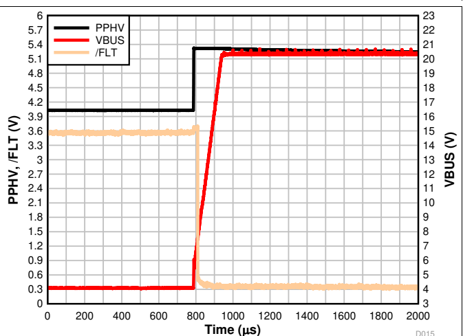
Figure 35. Fast Role Swap Response, 5-V Sink Contract, C_{VBUS} = 20 \mu F , I_{VBUS} = 0.5 A
