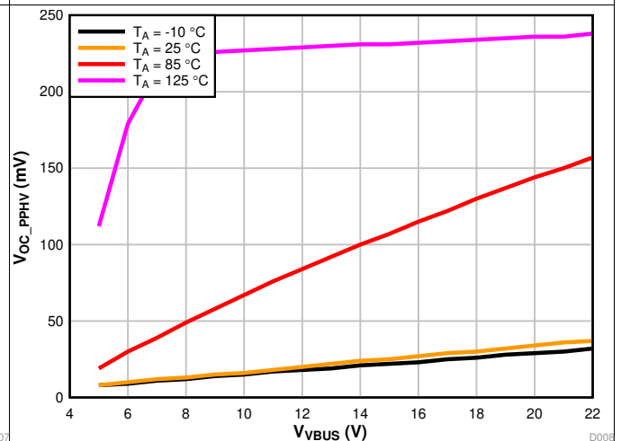
Figure 4. V_{OC\_PPHV} , PPHV Open Circuit Voltage versus VBUS
