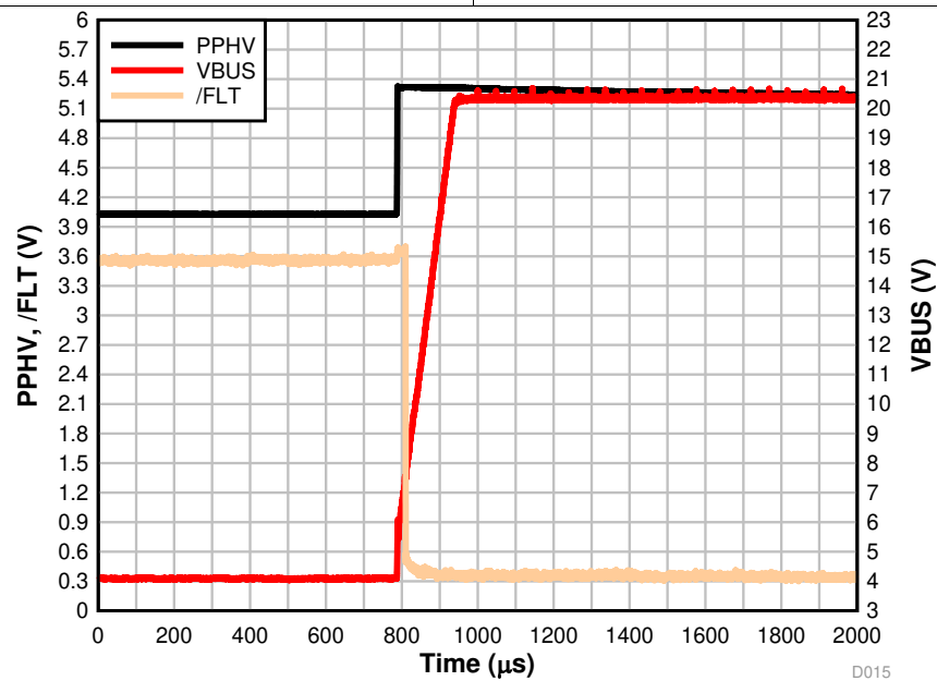
Figure 9. VBUS OVP Response with 6-V Threshold
