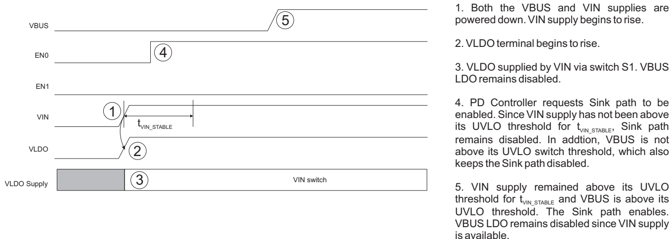
Figure 17. Normal Power Up Sequence
