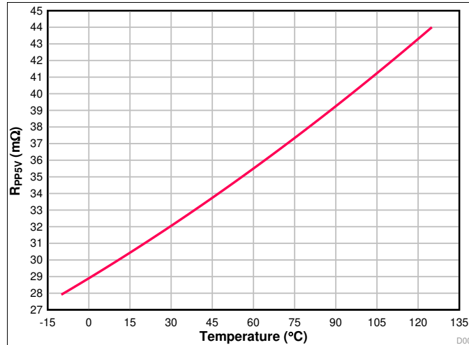
Figure 1. R_{PP5V} versus Temperature
