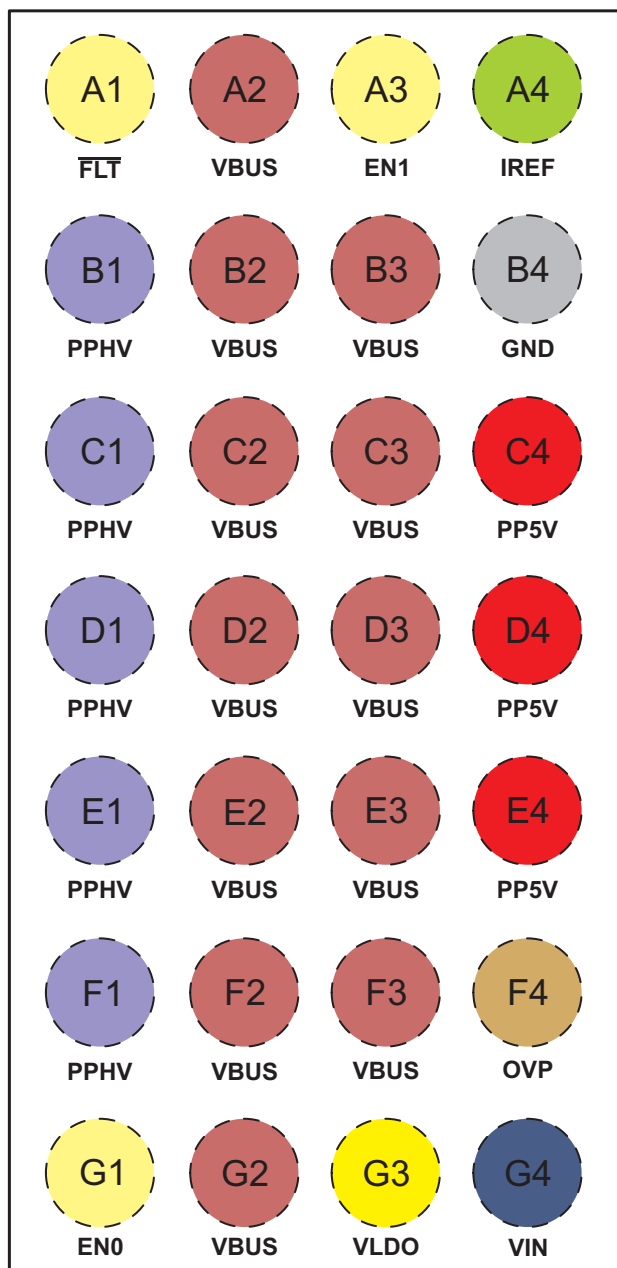
TPS6602x YBG Package 28-Pin WCSP Top View
