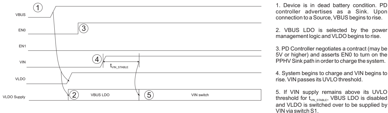
Figure 18. Dead Battery Power Up Sequence
