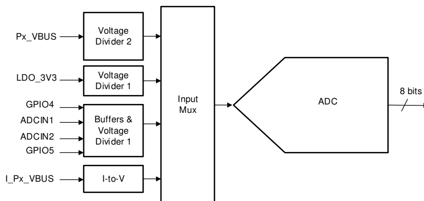
Figure 8-18. SAR ADC
