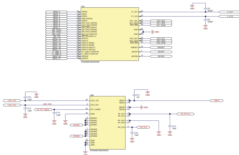
Figure 9-1. Example Schematic
