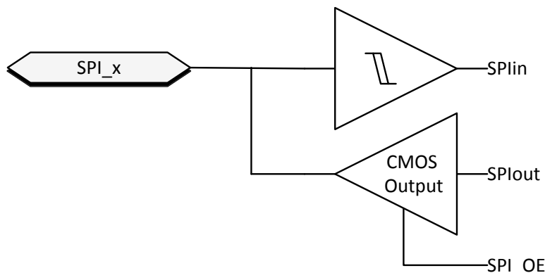
Figure 8-21. SPI buffer
