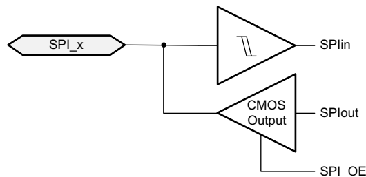
Figure 9-52. IOBUF_GPIOHSSI
