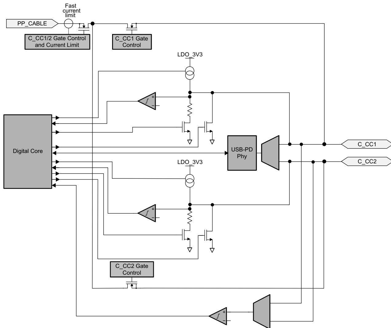
Figure 9-1. USB-PD Physical Layer and Simplified Plug and Orientation Detection Circuitry
