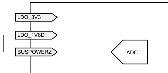
Figure 9-23. BUSPOWERZ Configured With PP_HV as Input Power Path
