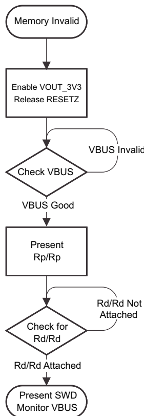
Figure 9-57. Memory Invalid Flow
