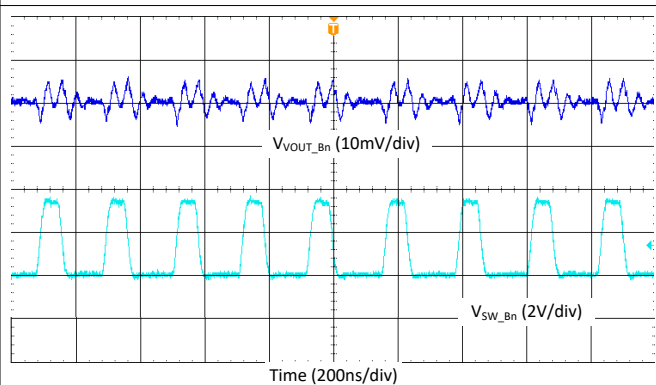
Figure 9-33. Buck Output Ripple - 4-Phase, Fsw = 4.4 MHz, Forced-PWM Mode
