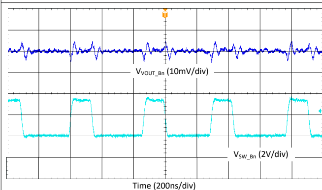
Figure 9-30. Buck Output Ripple - 3-Phase, Fsw = 4.4 MHz, Forced-PWM Mode
