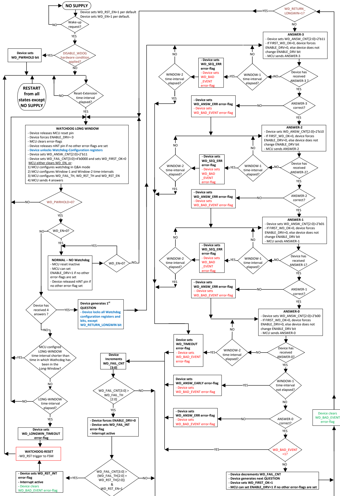
Figure 8-27. Flow Chart for WatchDog in Q&amp;A Mode
