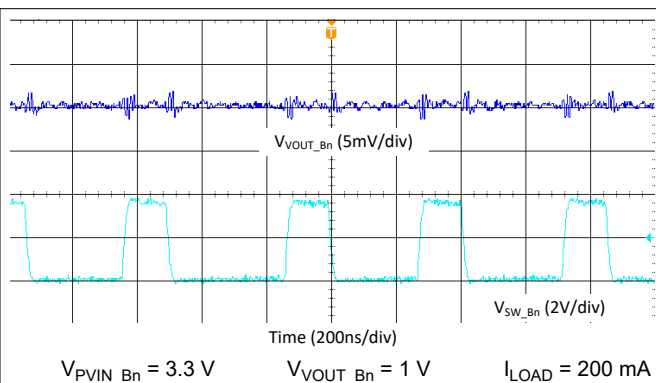
Figure 9-29. Buck Output Ripple - 3-Phase, Fsw = 2.2 MHz, Forced-PWM Mode
