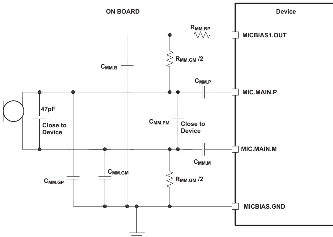
Figure 6-7. Analog Microphone Differential
