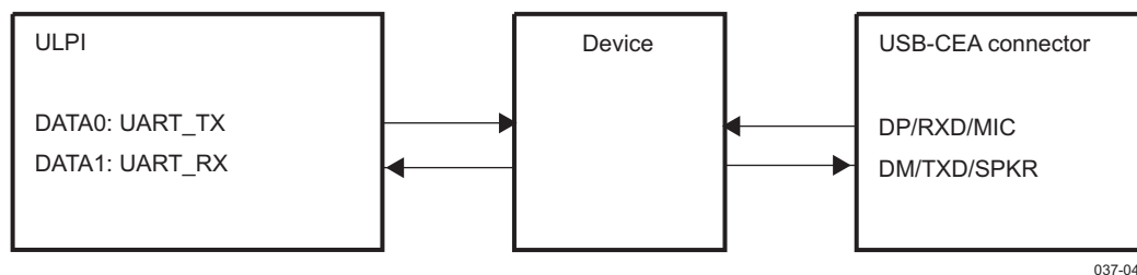
Figure 5-15. USB-CEA Carkit UART Data Flow
