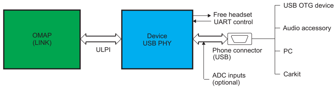
Figure 5-12. USB 2.0 PHY Block Diagram
