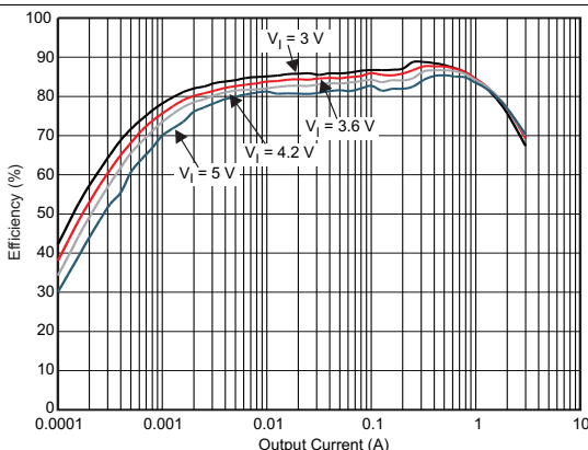
DCDC1 V_O = 1.1375\text{ V} DFE252012 PFM Mode 25°C
