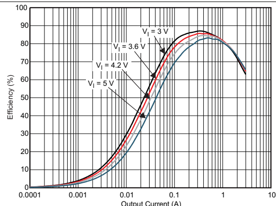
DCDC1 V_O = 0.9\text{ V} DFE252012 PWM Mode 25°C
