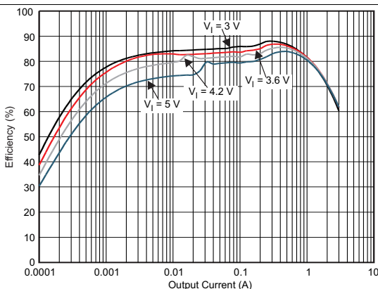
DCDC1 V_O = 1.2\text{ V} LQM2NPN-1 \mu\text{H} PFM Mode 25°C
