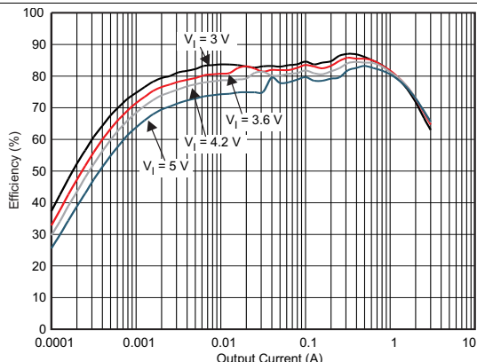
DCDC1 V_O = 0.9\text{ V} DFE252012 PFM Mode 25°C
