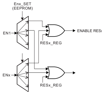
Figure 7-10. ENx Architecture
