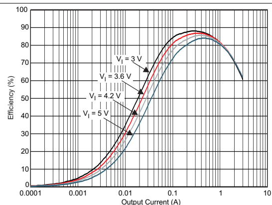
DCDC1 V_O = 1.2\text{ V} LQM2NPN-1 \mu\text{H} PWM Mode 25°C
