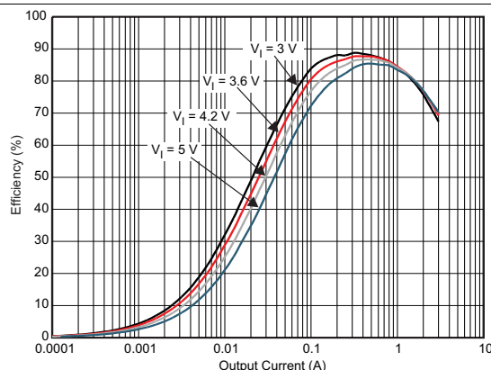
DCDC1 V_O = 1.1375\text{ V} DFE252012 PWM Mode 25°C
