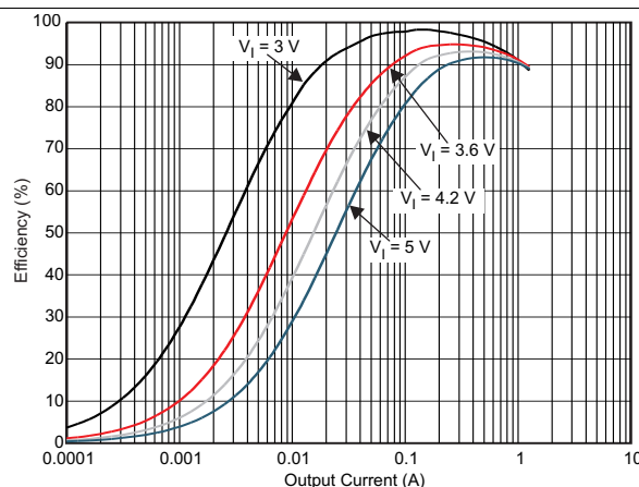
DCDC2 V_O = 2.95 V VLS201612-1 \mu H PFM Mode 25°C
