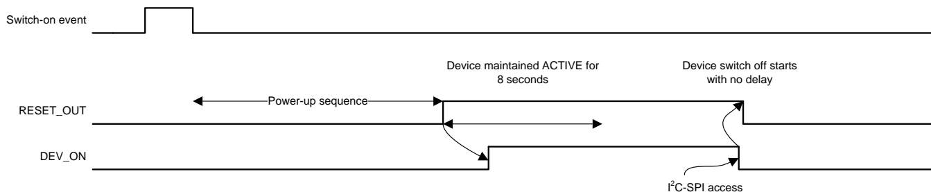
Figure 5-22. AUTODEVON Mode Timing Diagrams
