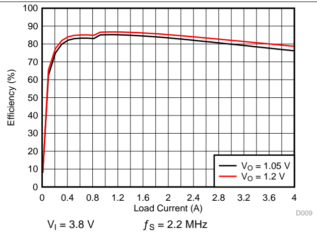
Figure 4-5. SMPS Efficiency for 4-A Multi-Phase PWM Mode
