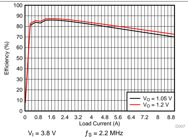
Figure 4-7. SMPS Efficiency for 9-A Multi-Phase PWM Mode
