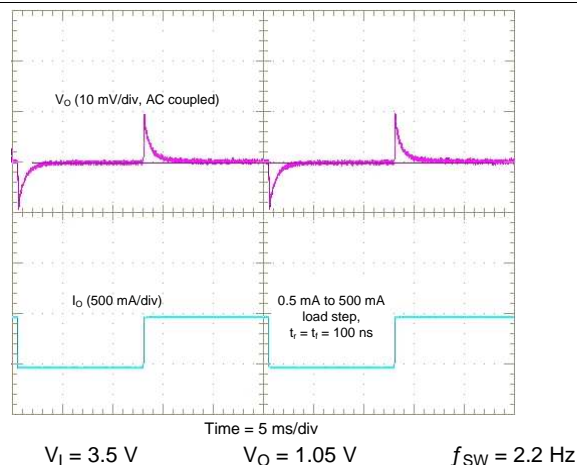
Figure 6-14. Typical SMPS Load Transient Response for SMPS12, SMPS3, SMPS45, SMPS6, and SMPS7
