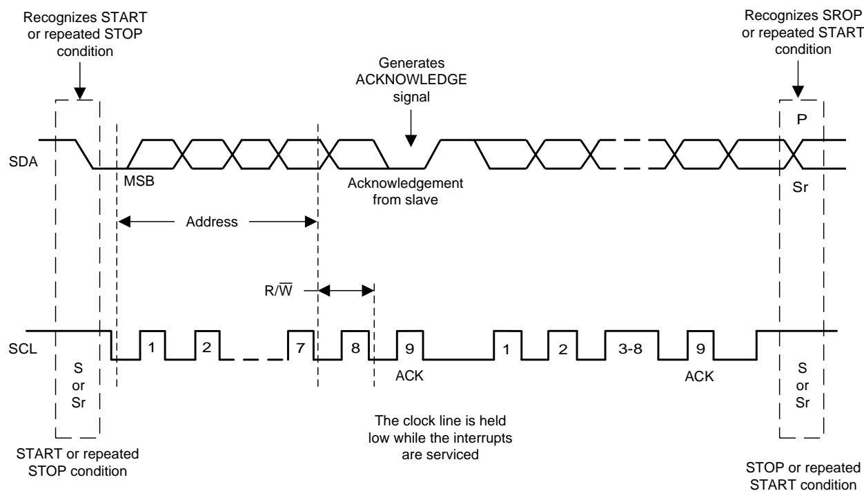
Figure 5-14. Bus Protocol
