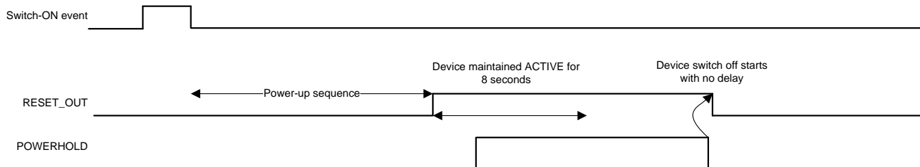
Figure 5-21. POWERHOLD Mode Timing Diagrams
