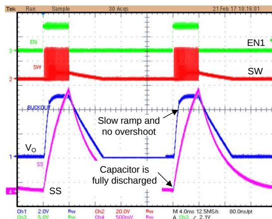
Figure 19. Passive Discharge With 2-MΩ Resistor
