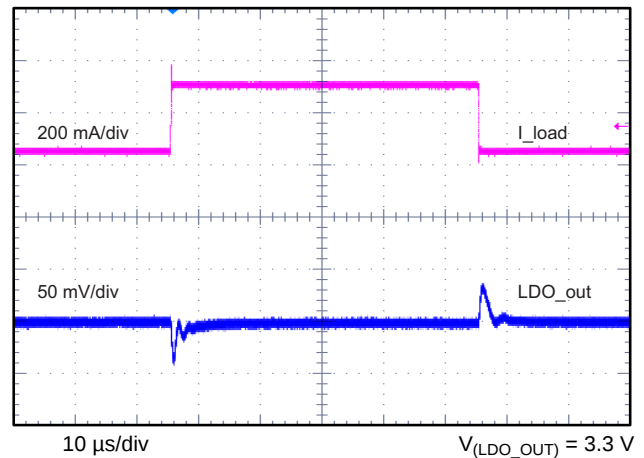
Figure 26. LDO-Regulator Output at Load Transient (50 mA to 300 mA)
