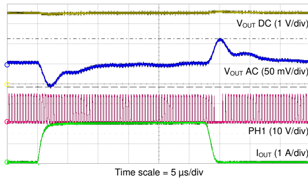
Figure 12-20. BOOST Load Regulation
