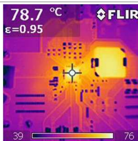
Figure 61. Thermal Signature of TPS65286EVM, T_A = \text{Room Temperature} , V_{IN} = 24\text{ V} , V_{OUT} = 5\text{ V}/5\text{ A} , I_{SW\_OUT1/2} = 0\text{ A} EVM Board: 4-Layer PCB, 1.6 mm Thickness, 2 oz. Copper Thickness, 65-mm x 65-mm Size, 25 Vias at Thermal Pad
