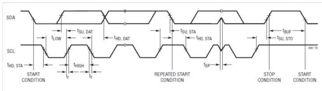
Figure 37. I 2 C Interface Timing Diagram
