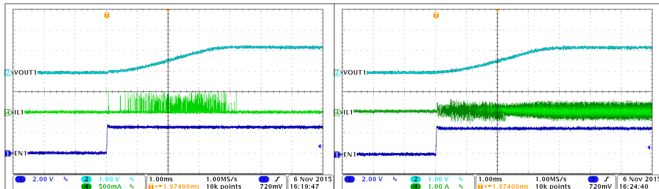
Figure 9-3. Buck1, PSM Mode, Soft-Start, I_{OUT} = 0\text{ A}
