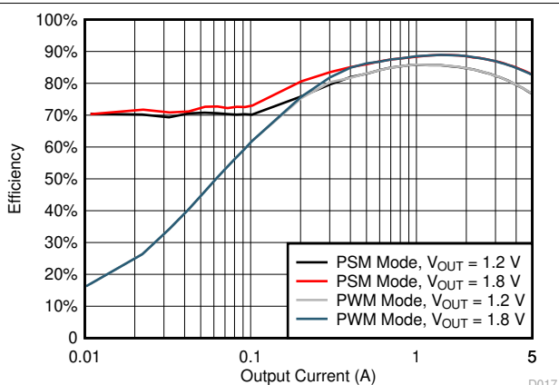
Figure 7-17. Buck1 Efficiency, V_{IN} = 12\text{ V} , F_{sw} = 610\text{ kHz}
