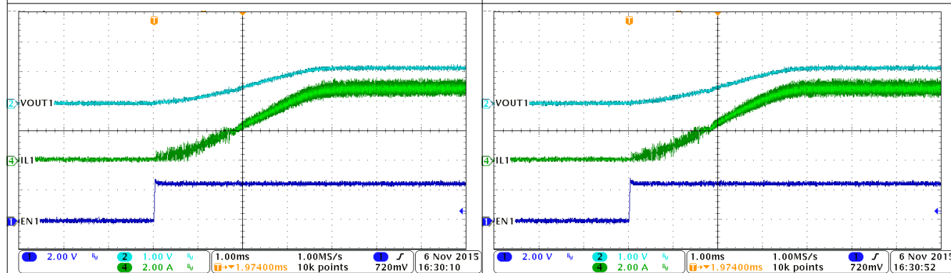
Figure 9-5. Buck1, PSM Mode, Soft-Start, I_{OUT} = 5\text{ A}
