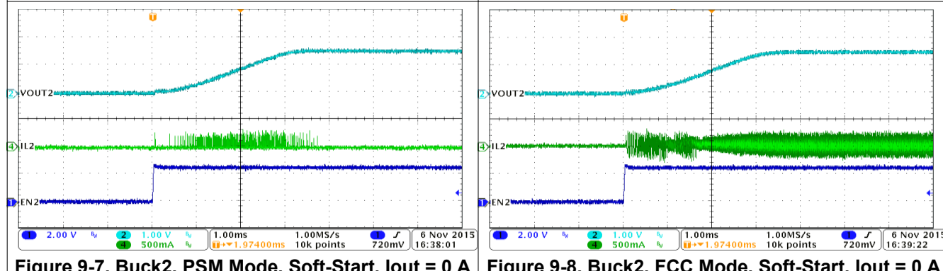
Figure 9-7. Buck2, PSM Mode, Soft-Start, I_{OUT} = 0\text{ A}
