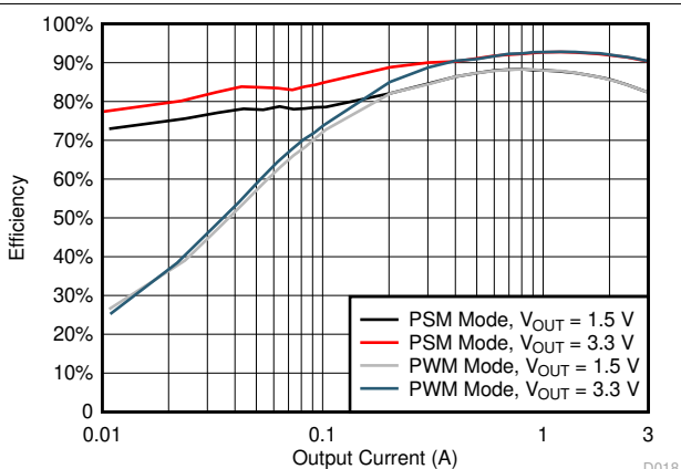
Figure 7-18. Buck2 Efficiency, V_{IN} = 12\text{ V} , F_{sw} = 610\text{ kHz}
