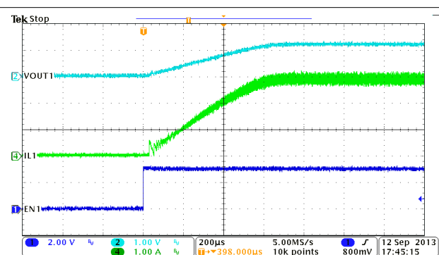
Figure 9-3. BUCK1, Soft-Start With Full Load
