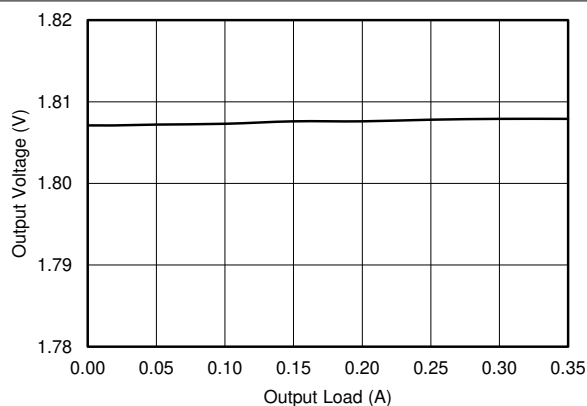
Figure 7-9. LDO1, Load Regulation
