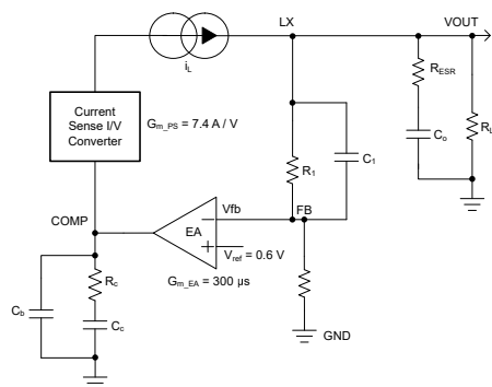
Figure 9-1. DC/DC Loop Compensation
