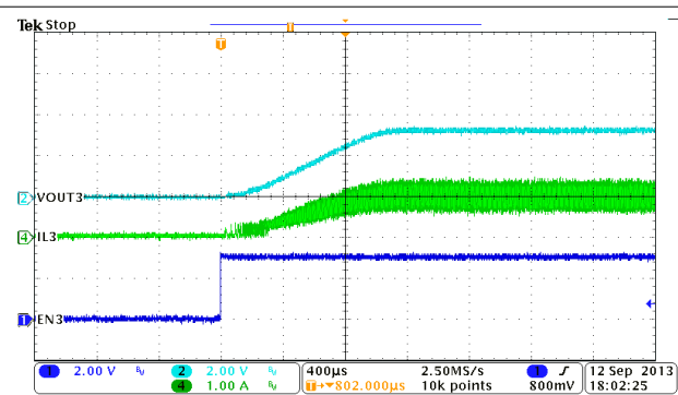
Figure 9-7. BUCK3, Soft-Start With Full Load
