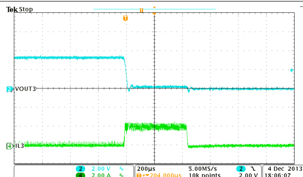
Figure 9-24. Buck3, OCP
