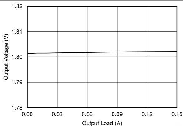
Figure 7-10. LDO2, Load Regulation
