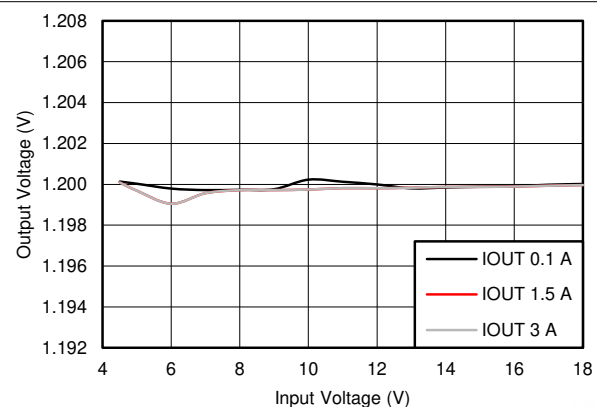
Figure 7-6. BUCK1, Line Regulation
