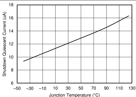
Figure 7-15. Shutdown Quiescent Current vs Temperature
