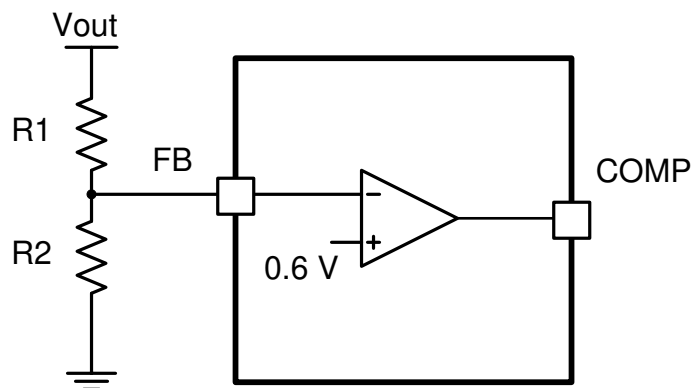
Figure 8-1. Voltage Divider Circuit
