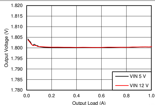
Figure 7-4. BUCK2, Load Regulation
