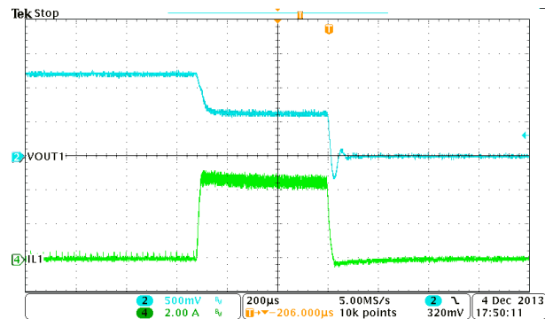
Figure 9-20. Buck1, OCP
