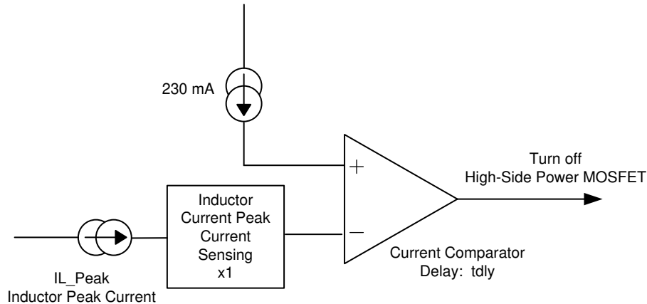
Figure 8-6. PSM Current Comparator
