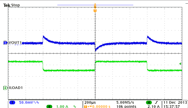
Figure 9-15. Buck1, Load Transient, 1.5 to 2.25 A SR = 0.25 A/µs
