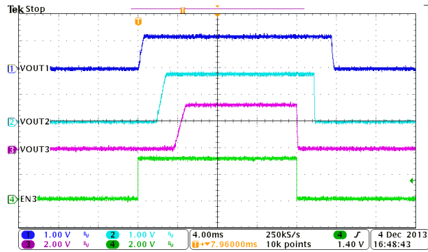
Figure 9-26. Automatic Power Sequencing, MODE = EN1 = EN2 = HIGH
