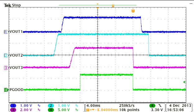
Figure 9-31. Automatic Power Sequencing, MODE = EN2 = HIGH, EN1 = LOW
