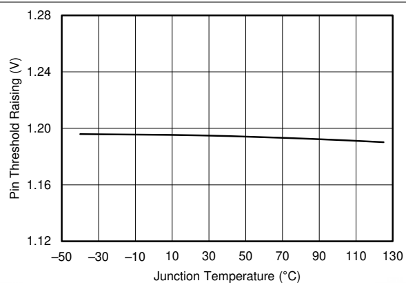
Figure 7-18. EN Pin Threshold Rising vs Temperature
