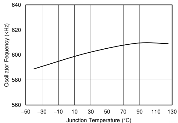
Figure 7-14. Oscillator Frequency vs Temperature
