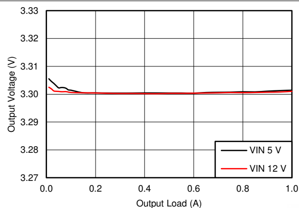
Figure 7-5. BUCK3, Load Regulation
