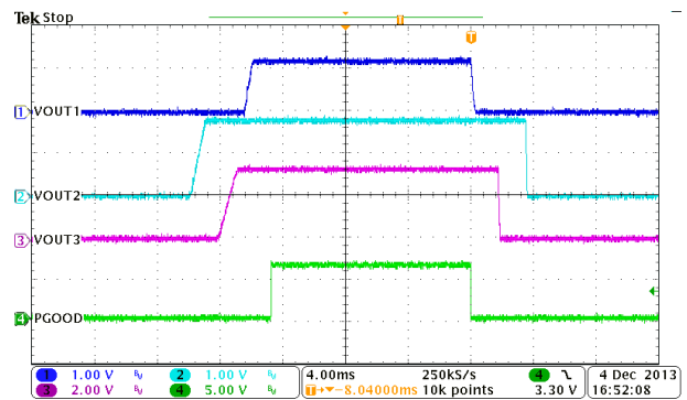
Figure 9-29. Automatic Power Sequencing, MODE = EN1 = HIGH, EN2 = LOW
