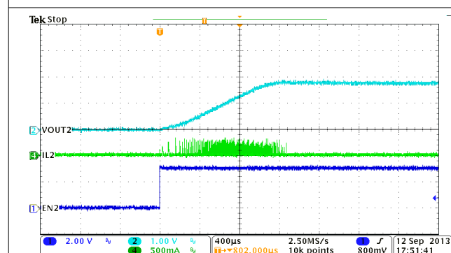
Figure 9-4. BUCK2, Soft-Start With No Load
