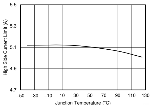
Figure 7-21. Buck1 High-Side Current Limit vs Temperature
