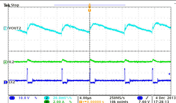
Figure 9-10. Buck2, Steady State Operation at Light Load
