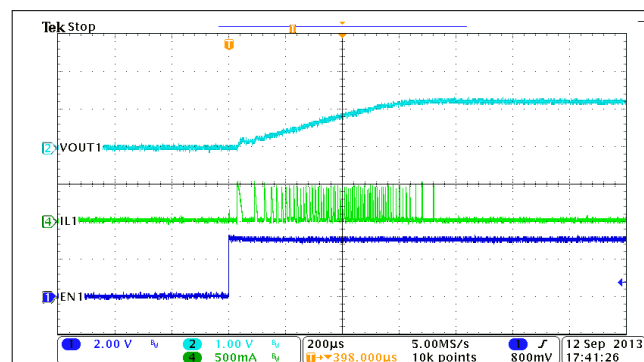
Figure 9-2. BUCK1, Soft-Start With No Load
