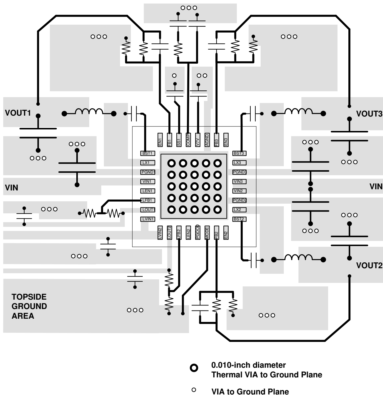
Figure 9-34. PCB Layout
