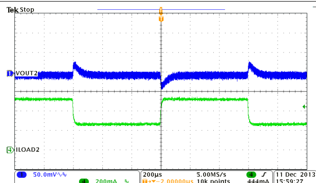
Figure 9-16. Buck2, Load Transient, 0.25 to 0.5 A SR = 0.25 A/µs
