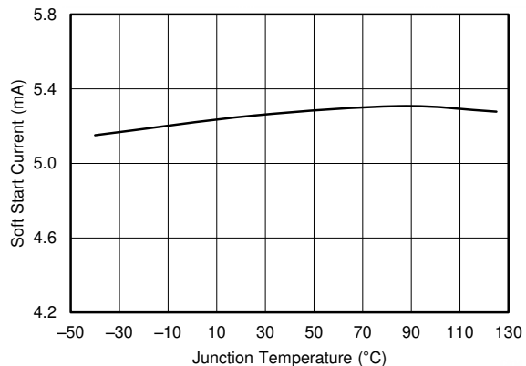
Figure 7-20. SS Pin Charge Current vs Temperature
