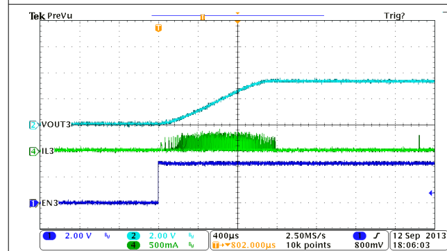
Figure 9-6. BUCK3, Soft-Start With No Load
