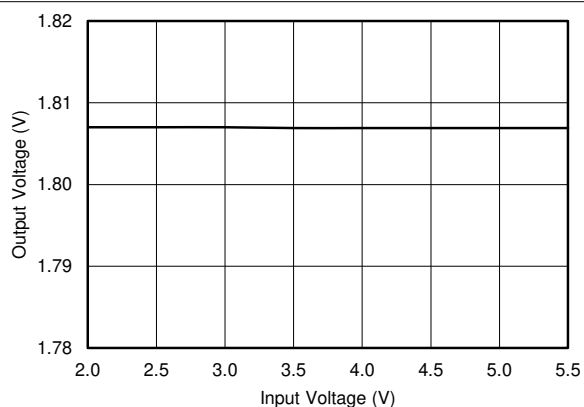
Figure 7-11. LDO1, Line Regulation
