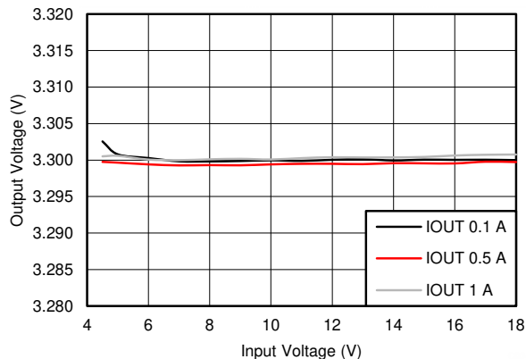
Figure 7-8. BUCK3, Line Regulation
