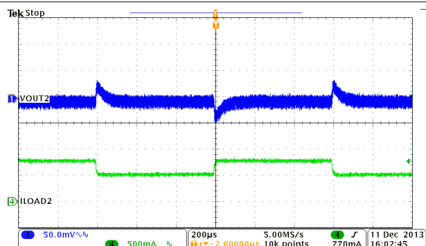
Figure 9-17. Buck2, Load Transient, 0.5 to 0.75 A SR = 0.25 A/µs
