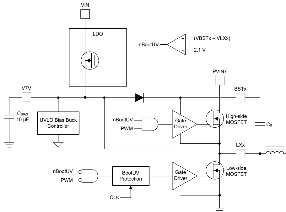
Figure 8-5. V7V Linear Dropout Regulator and Bootstrap Voltage Diagram
