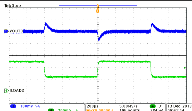
Figure 9-18. Buck3, Load Transient, 0.25 to 0.5 A SR = 0.25 A/µs
