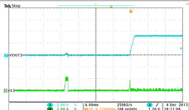
Figure 9-25. Buck3, Hiccup and Recovery
