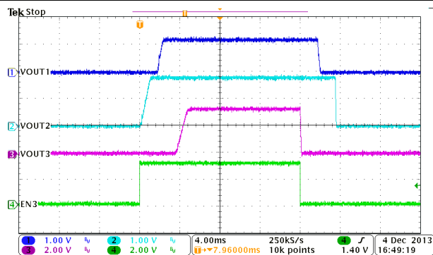
Figure 9-30. Automatic Power Sequencing, MODE = EN2 = HIGH, EN1 = LOW
