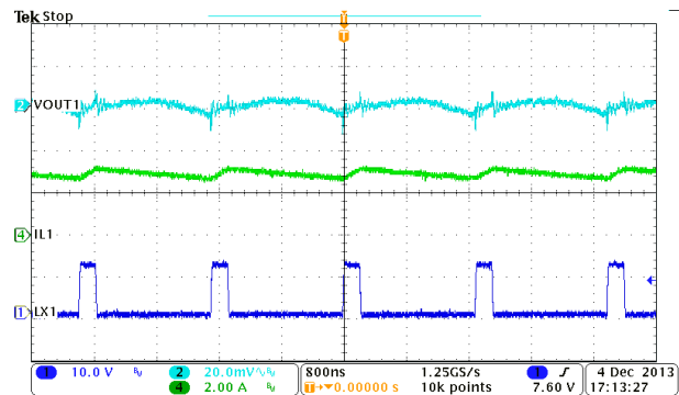
Figure 9-9. Buck1, Steady State Operation at Full Load
