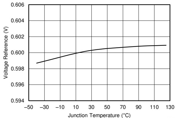
Figure 7-13. Voltage Reference vs Temperature
