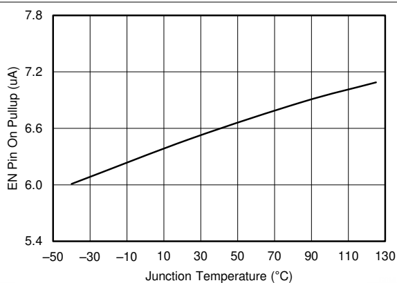
Figure 7-17. EN Pin Pullup Current vs Temperature, EN = 1.5 V
