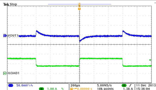
Figure 9-14. Buck1, Load Transient, 0.75 to 1.5 A SR = 0.25 A/µs
