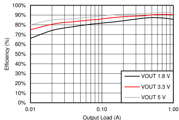
Figure 7-2. BUCK2 Efficiency
