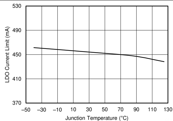
Figure 7-23. LDO Current Limit vs Temperature
