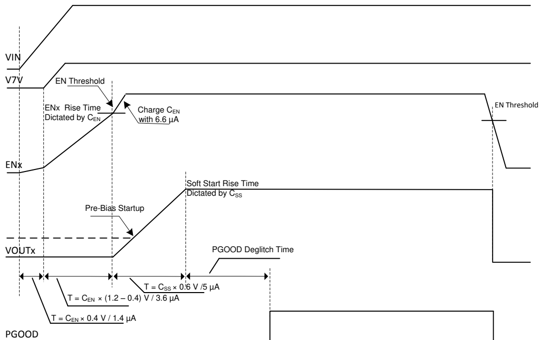
Figure 8-3. Startup Power Sequence
