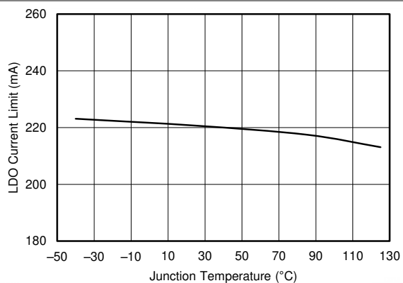
Figure 7-24. LDO2 Current Limit vs Temperature
