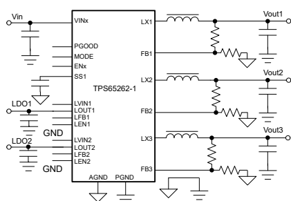
Typical Application
