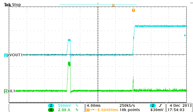
Figure 9-21. Buck1, Hiccup and Recovery
