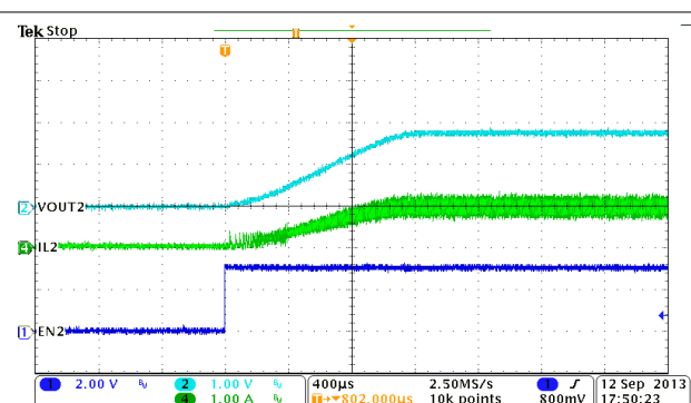
Figure 9-5. BUCK2, Soft-Start With Full Load
