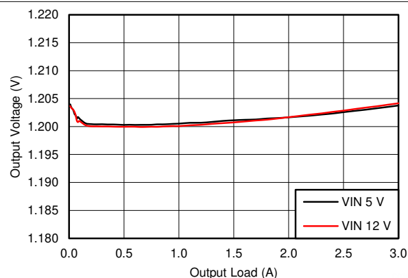
Figure 7-3. BUCK1, Load Regulation
