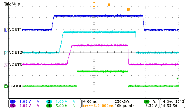
Figure 9-27. Automatic Power Sequencing, MODE = EN1 = EN2 = HIGH
