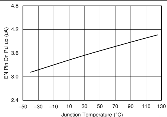
Figure 7-16. EN Pin Pullup Current vs Temperature, EN = 1 V
