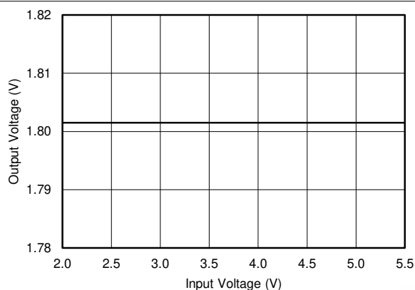
Figure 7-12. LDO2, Line Regulation
