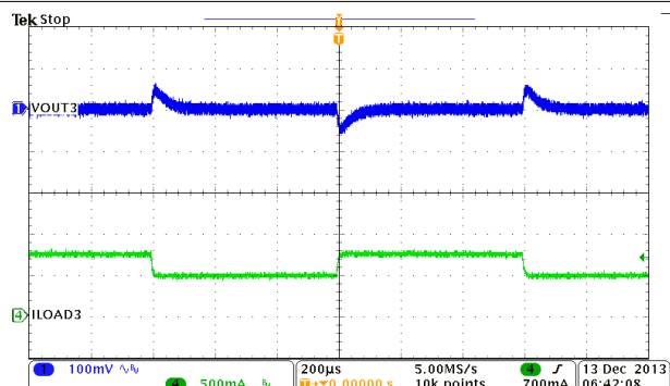
Figure 9-19. Buck3, Load Transient, 0.5 to 0.75 A SR = 0.25 A/µs
