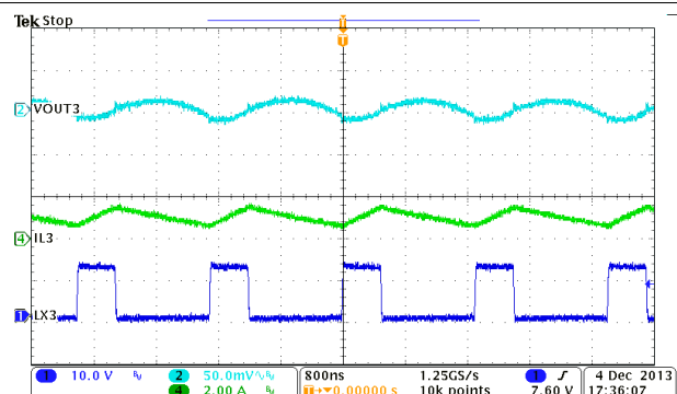
Figure 9-13. Buck3, Steady State Operation at Full Load
