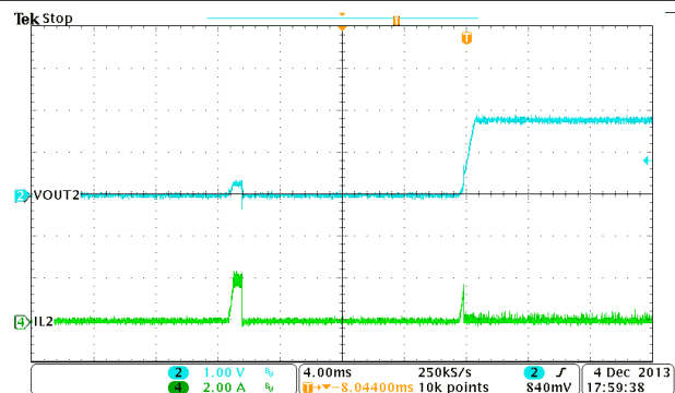
Figure 9-23. Buck2, Hiccup and Recovery
