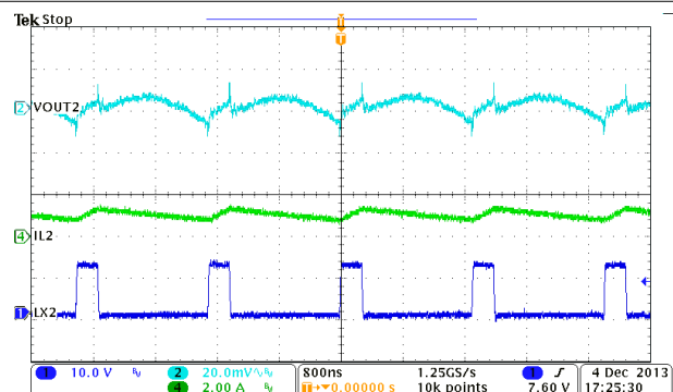
Figure 9-11. Buck2, Steady State Operation at Full Load
