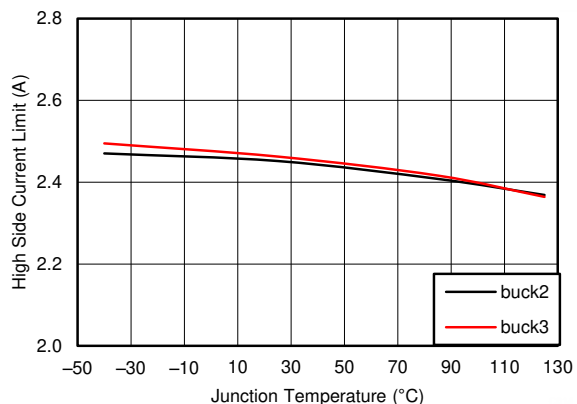
Figure 7-22. Buck2, 3 High-Side Current Limit vs Temperature
