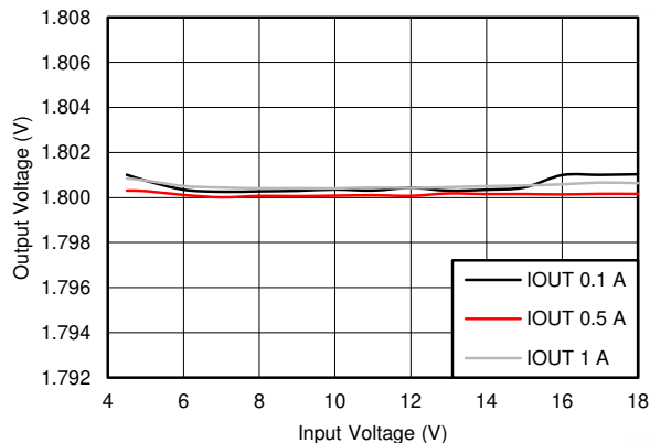
Figure 7-7. BUCK2, Line Regulation
