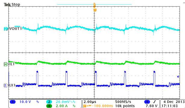
Figure 9-8. Buck1, Steady State Operation at Light Load
