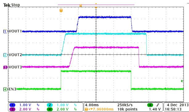
Figure 9-28. Automatic Power Sequencing, MODE = EN1 = HIGH, EN2 = LOW
