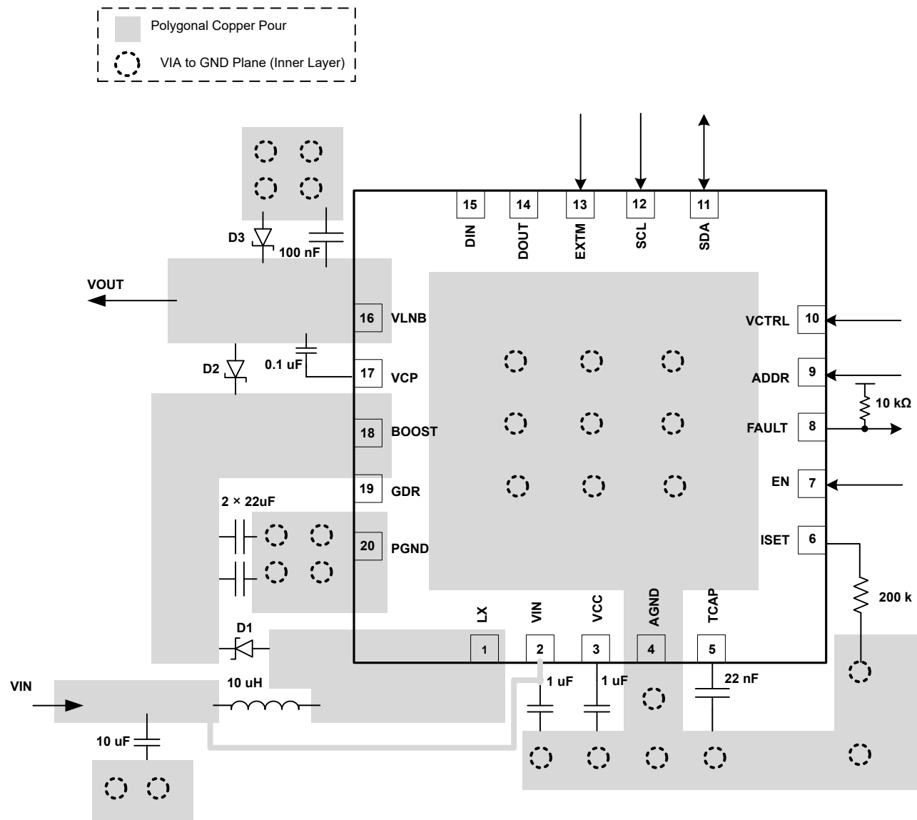
Figure 8-22. Layout
