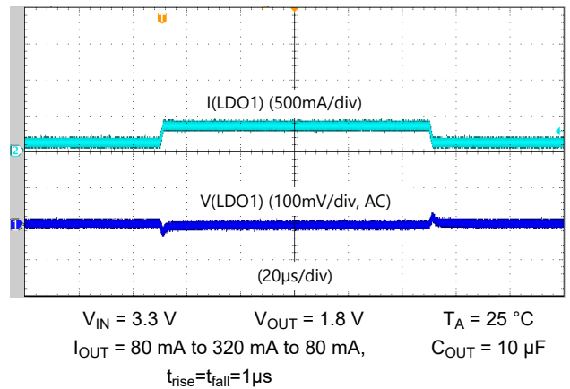
Figure 5-6. LDO1 Load-step response
