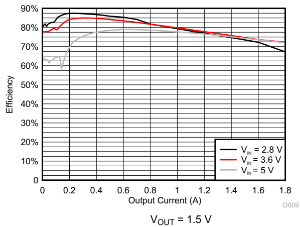
Figure 8-5. DCDC3 Efficiency
