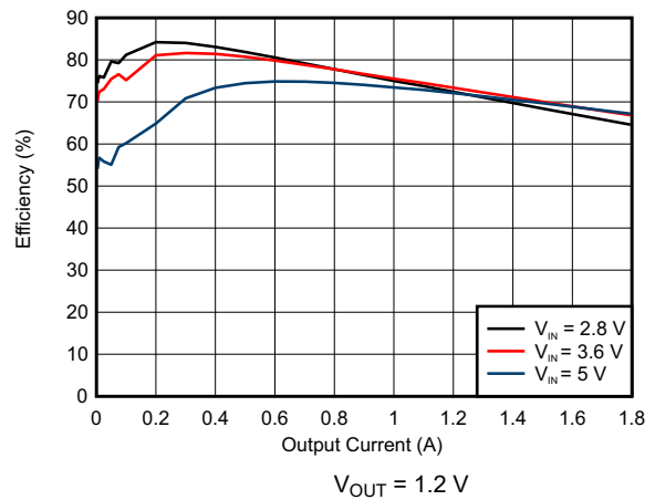
Figure 8-5. DCDC3 Efficiency
