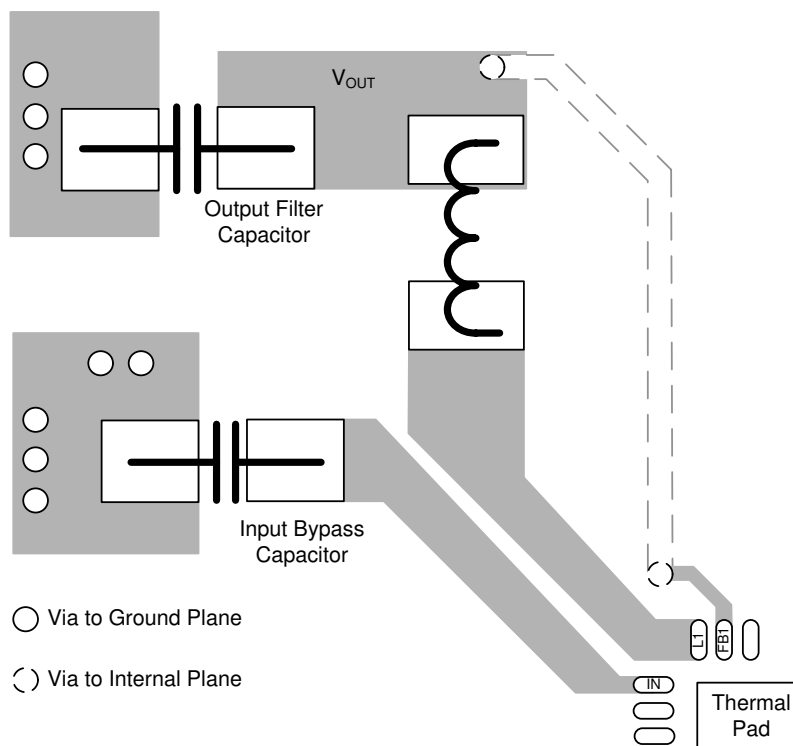
Figure 10-1. Layout Recommendation
