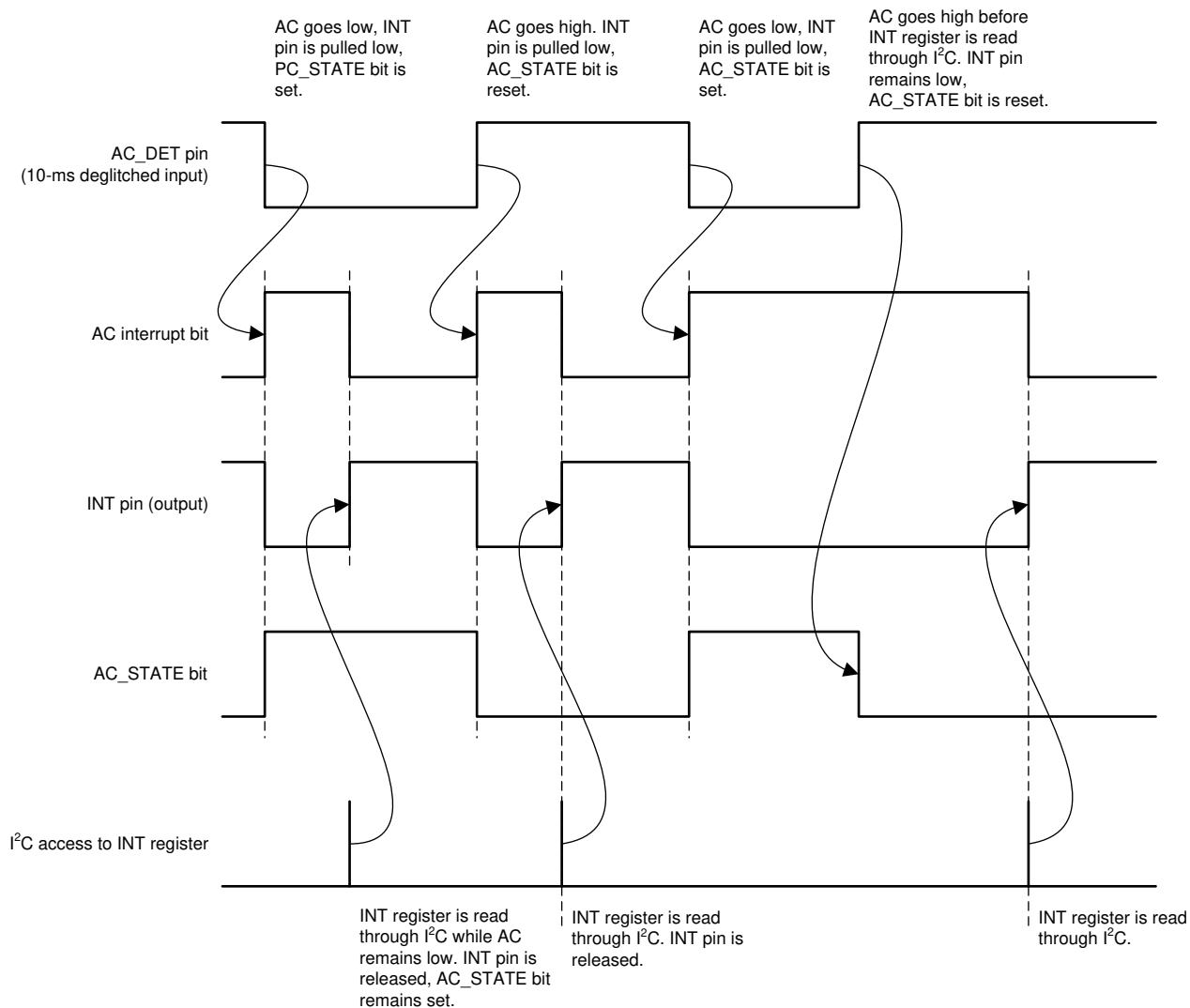
Figure 7-29. AC_STATE Pin
