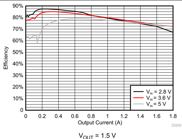
Figure 8-6. DCDC3 Efficiency
