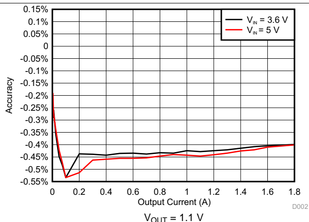
Figure 4-2. DCDC2 Accuracy
