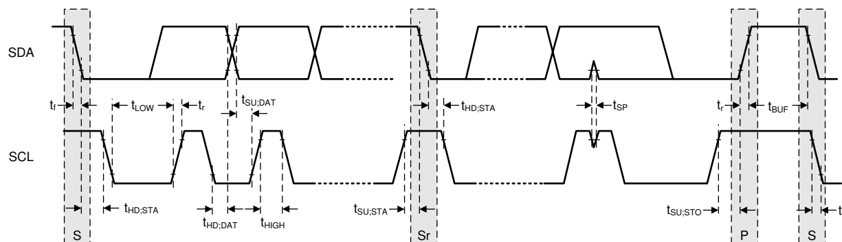
Figure 5-23. I²C Protocol and Transmission Timing I²C Data Transmission Timing
