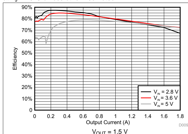
Figure 6-4. DCDC3 Efficiency
