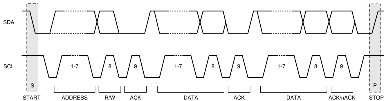
Figure 5-22. I²C Protocol and Transmission Timing I²C Start Stop and Acknowledge Protocol
