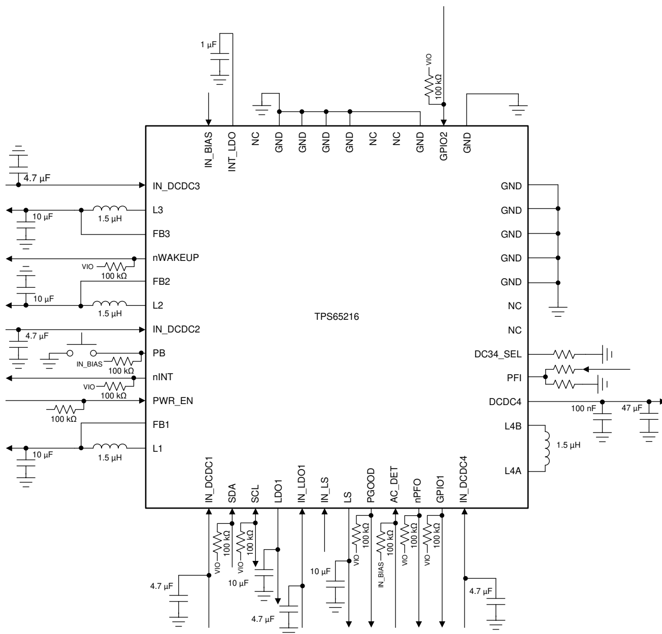
Figure 1-1. Simplified Schematic
