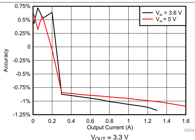
Figure 4-4. DCDC4 Accuracy
