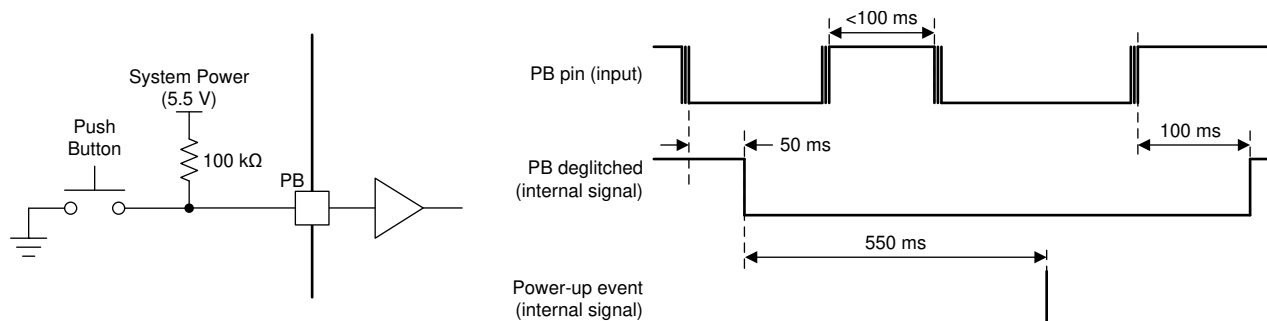
Figure 5-15. Left: Typical PB Input Circuit Right: Push-Button Input (PB) Deglitch and Power-Up Timing
