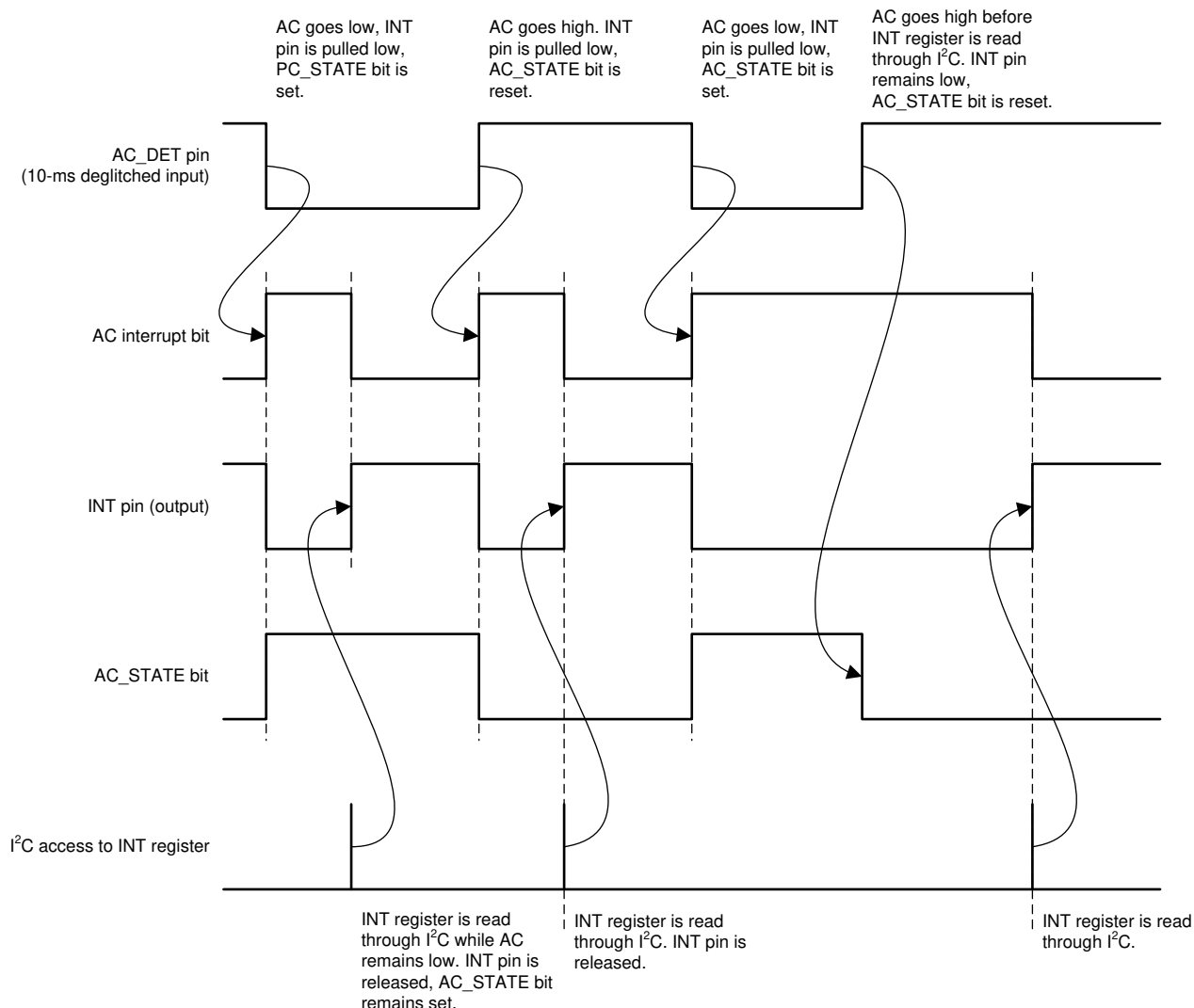
Figure 5-19. AC_STATE Pin
