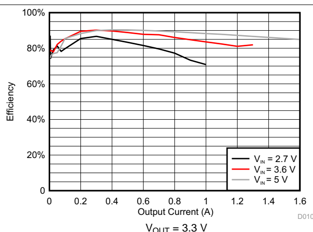
Figure 6-5. DCDC4 Efficiency
