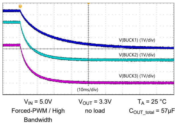
Figure 7-8. Bucks Discharge
