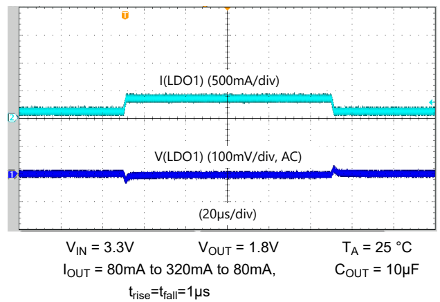
Figure 5-6. LDO1 Load-step Response
