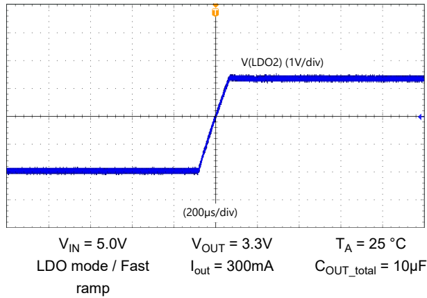
Figure 7-6. LDO2 Fast Ramp
