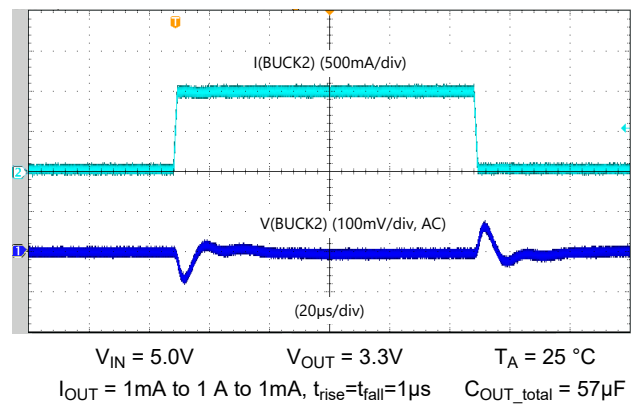
Figure 5-4. BUCK2 Load-step Response - Low Bandwidth, Forced PWM
