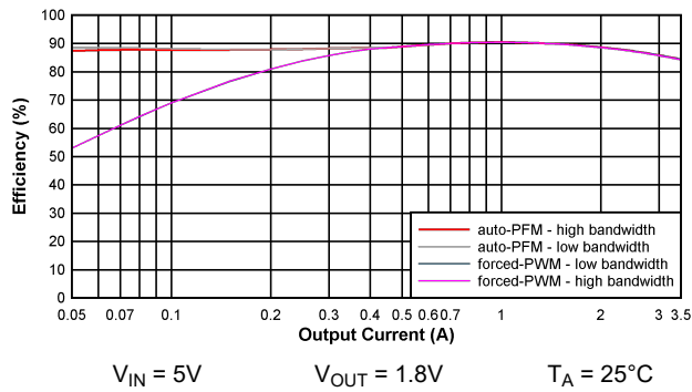
Figure 5-1. Efficiency BUCK1
