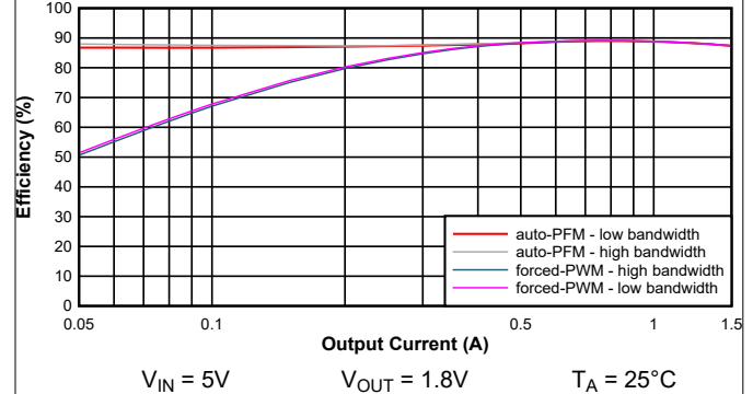
Figure 5-2. Efficiency BUCK23
