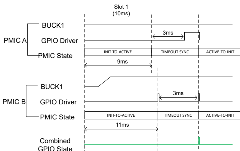
Figure 6-17. Timeout Synchronization
