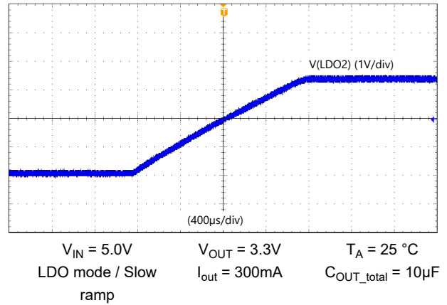
Figure 7-7. LDO2 Slow Ramp
