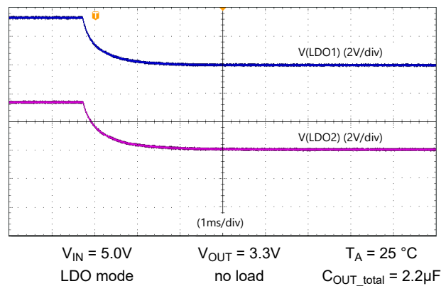
Figure 7-9. LDOs Discharge
