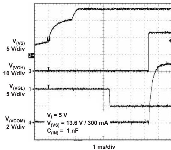
Figure 26. Power-On Sequencing
