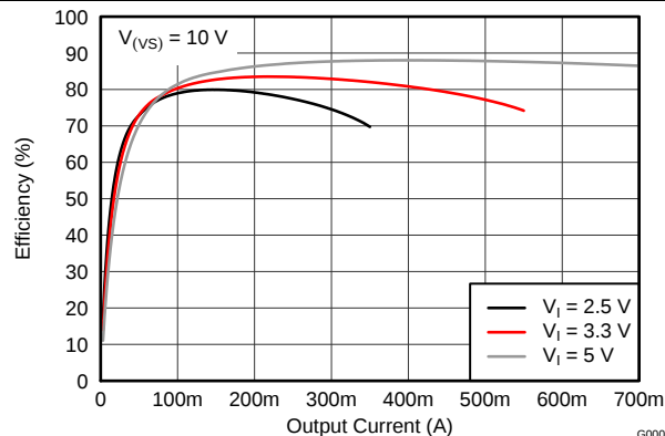
Figure 18. Boost Converter Efficiency ( V_{(VS)} = 10 \text{ V} )
