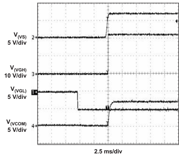
Figure 27. Power-On Sequencing With External Isolation MOSFET
