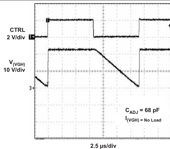
Figure 28. Gate Voltage Shaping
