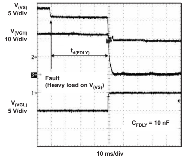
Figure 29. Adjustable Fault Detection Time
