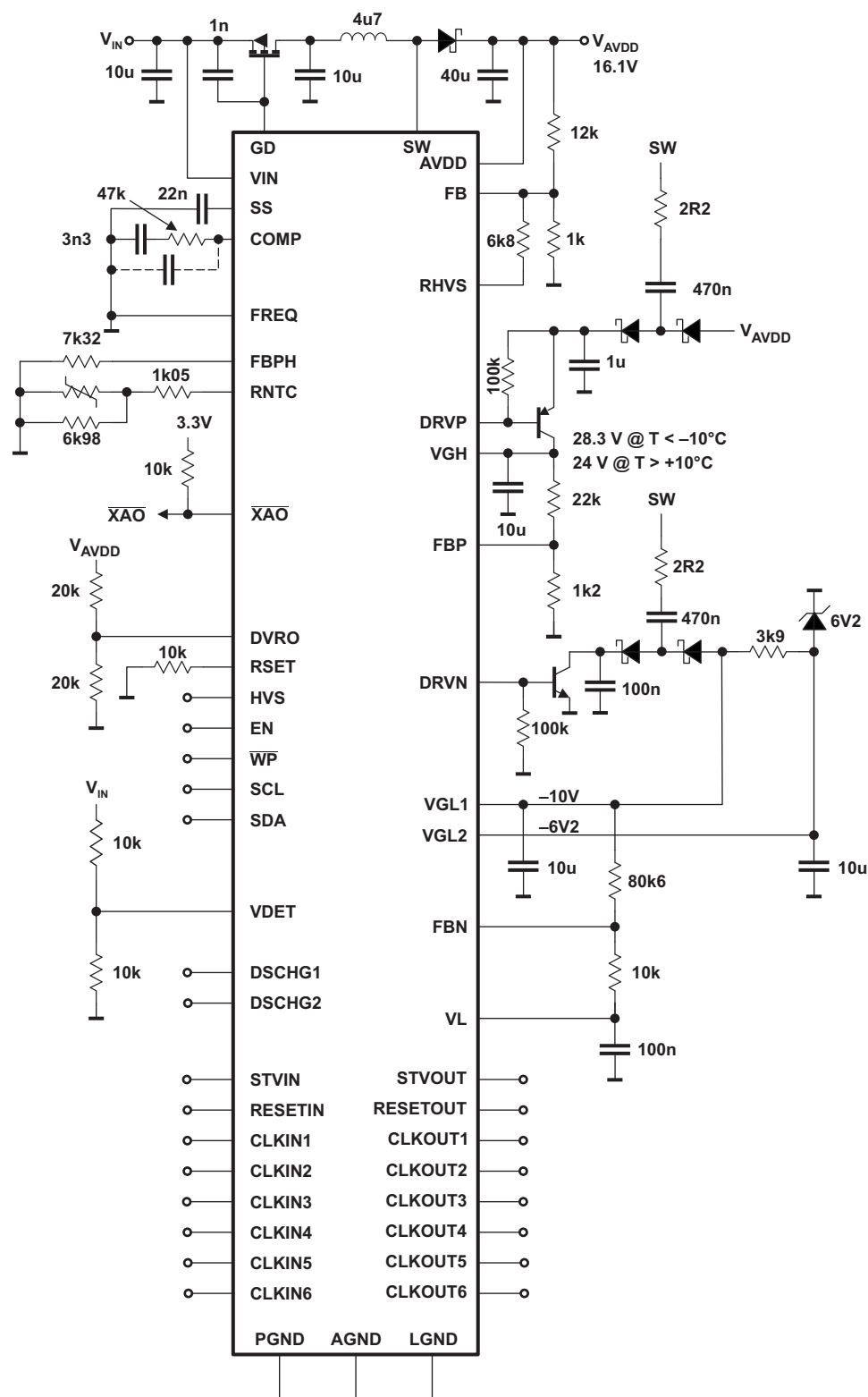
Figure 51. Typical Application Circuit Using Positive Charge Pump in ×2 Configuration
