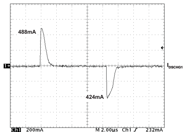
PEAK OUTPUT CURRENT (DSCHRGx)
