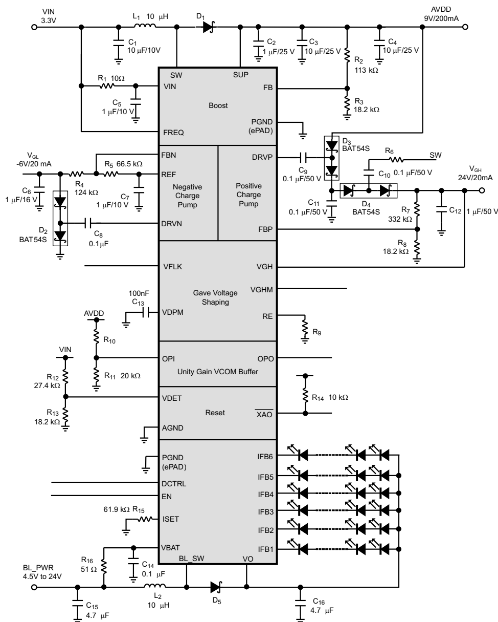
Figure 33. Typical Application Circuit
