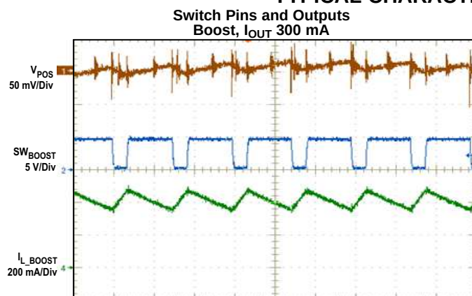
400 ns/div Figure 5.
