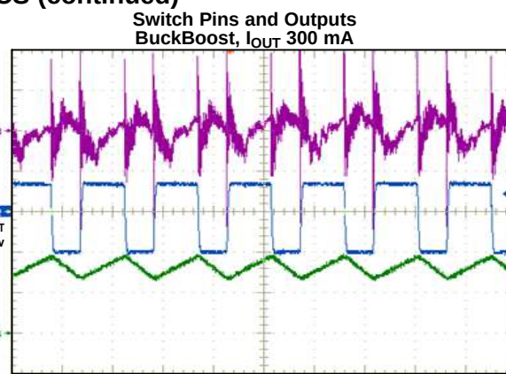
400 ns/div Figure 6.
