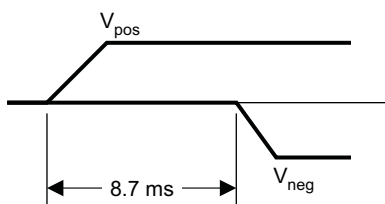
Figure 15. Start-Up Sequencing
