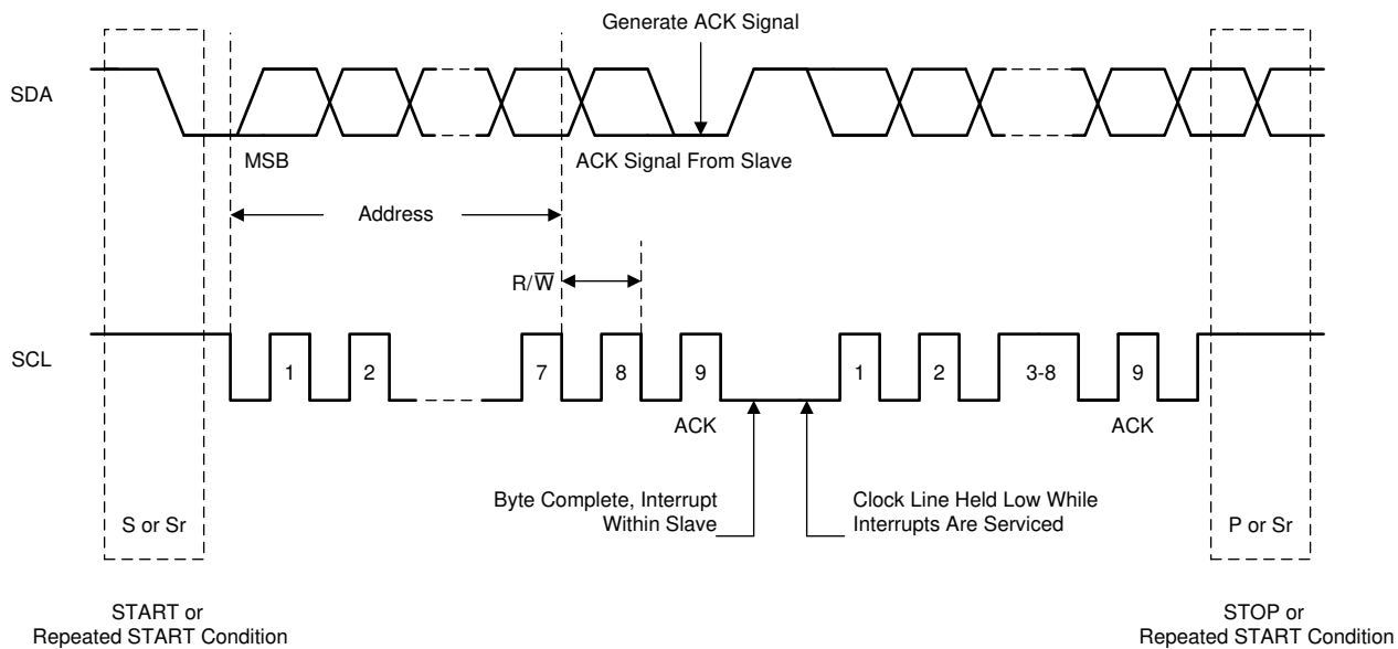
Figure 6-12. I²C Bus Protocol
