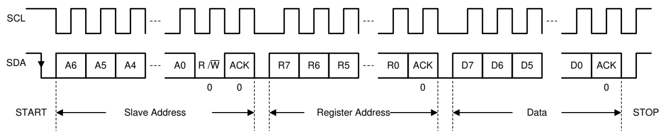
Figure 6-13. I²C Interface WRITE to TPS6508700 in F/S Mode
