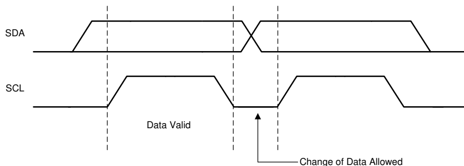
Figure 6-10. Bit Transfer on the I²C Bus
