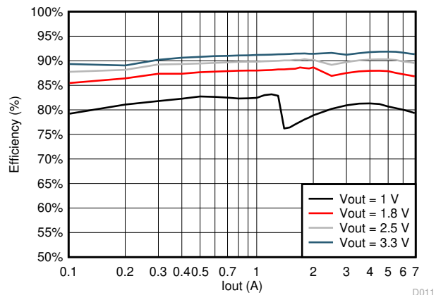
Figure 5-3. BUCK6 Efficiency at V_{IN} = 13V
