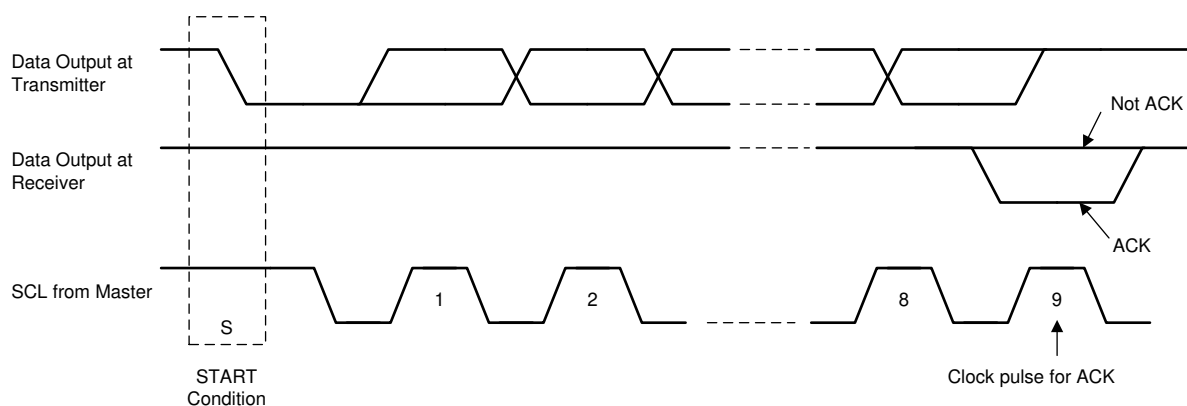
Figure 6-11. Acknowledge on the I²C Bus
