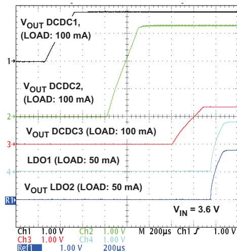
Figure 20. Startup DCDC1, DCDC2, AND DCDC3, LDO1, LDO2
